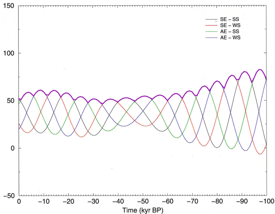
Fig. 4. Time evolution over the last 100 kyr of the amplitude of the 24-h mean irradiance at the equator between spring equinox and summer solstice (black), spring equinox and winter solstice (red), autumn equinox and summer solstice (green) and autumn equinox and winter solstice (blue), and the largest amplitude in the seasonal cycle (purple). Units are \text{Wm}^{-2} .
