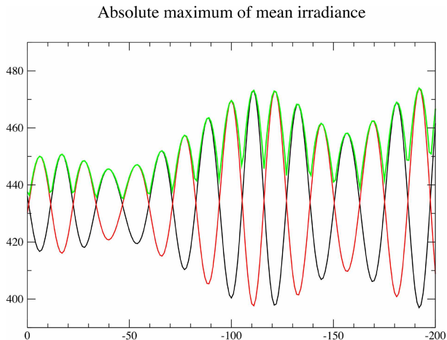
Fig. 2. Time evolution over the last 200 kyr of the 24-h mean irradiance at the equator at spring equinox (black curve) and at autumn equinox (red curve). The time evolution of the maximum of these two series is drawn in green. Units are \text{Wm}^{-2} .
