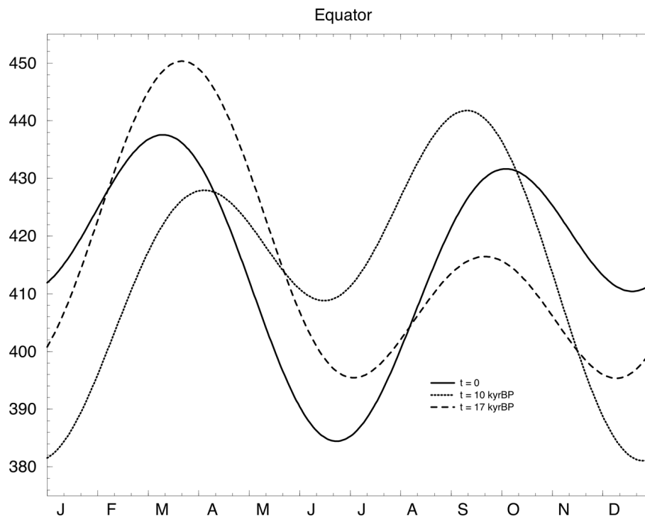
Fig. 1. Seasonal cycle of insolation at the equator at present (full line), at 10 kyr BP (dotted line) and at 17 kyr BP (dashed line). Units are Wm^{-2} .
