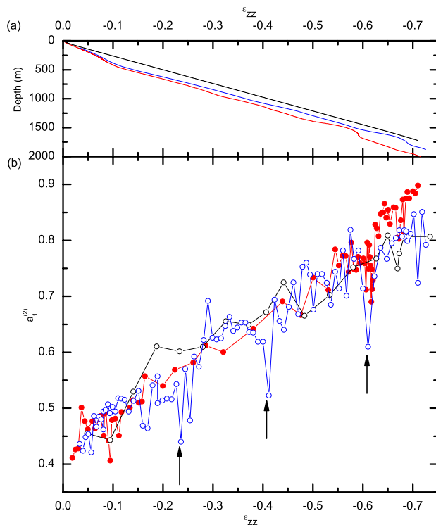
Fig. 2. (a) Evolution of depth as a function of the cumulative strain \epsilon_{zz} , along the EDC (red lines), DF (Blue line) and GRIP (black line) cores. This corresponds to the thinning function as calculated by the current dating models (Parrenin et al., 2006b 2 ; Johnsen and Dansgaard, 1992). (b) Evolution of a_1^{(2)} as a function of \epsilon_{zz} experienced by the considered layer for the EDC (red circles), DF (open blue circles) and GRIP cores (open black circles).
