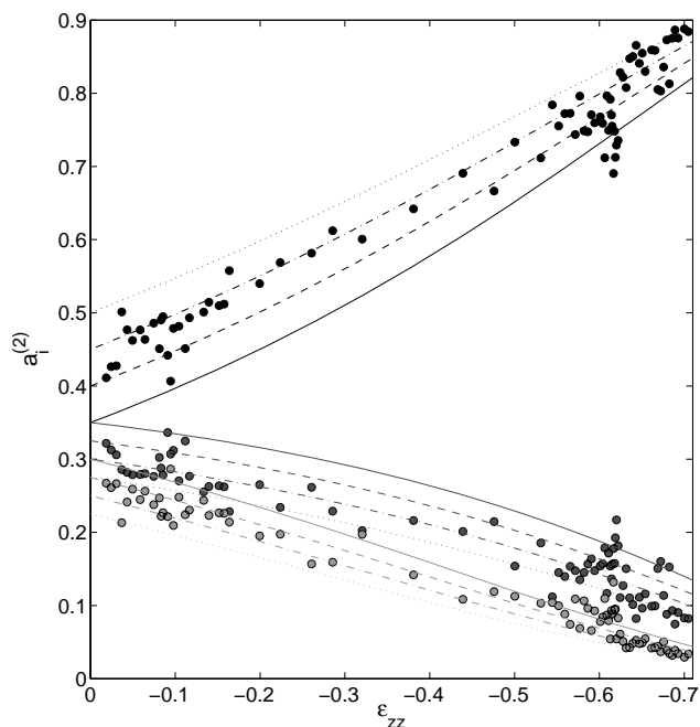
Fig. 3. Evolution of the eigenvalues of a^{(2)} as a function of \epsilon_{zz} along the EDC core: a_1^{(2)} in black, a_2^{(2)} in gray and a_3^{(2)} in light gray. Close symbols corresponds to the data, whereas lines show the outputs of the model for different initial fabrics (a_1^{(2)}, a_2^{(2)}, a_3^{(2)}) : (0.35, 0.35, 0.30) continuous line, (0.40, 0.325, 0.275) dashed line, (0.45, 0.30, 0.25) dashed-dotted line, (0.50, 0.275, 0.225) dotted line.
