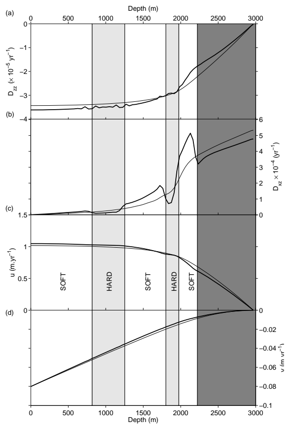
Fig. 6. Evolution with depth in an ice core situated at 30 km from the ice divide of: (a) the longitudinal strain-rate D_{zz} , (b) the shear strain-rate D_{xz} , (c) the horizontal velocity u and (d) the vertical velocity v .
