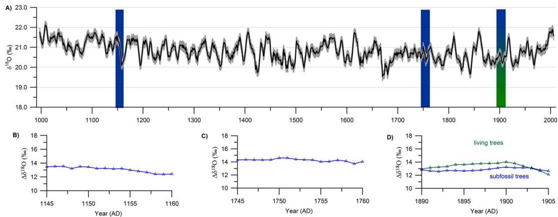
Fig. 1. Figure IV. (A) Millennial \delta^{18}\text{O} series with box corresponding to the period where D\delta^{18}\text{O} values have been calculated. The calculated D\delta^{18}\text{O} values for the (B) 1145–1160, (C) 1745–1760, and (D) 1890–1905
