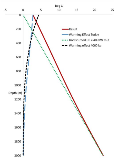
Fig. 2. Subsurface temperature model results based on the surface temperature depicted in Figure 1. The dotted green line shows an undisturbed temperature profile with heat flow at 40 mW m-2. The long-dash
