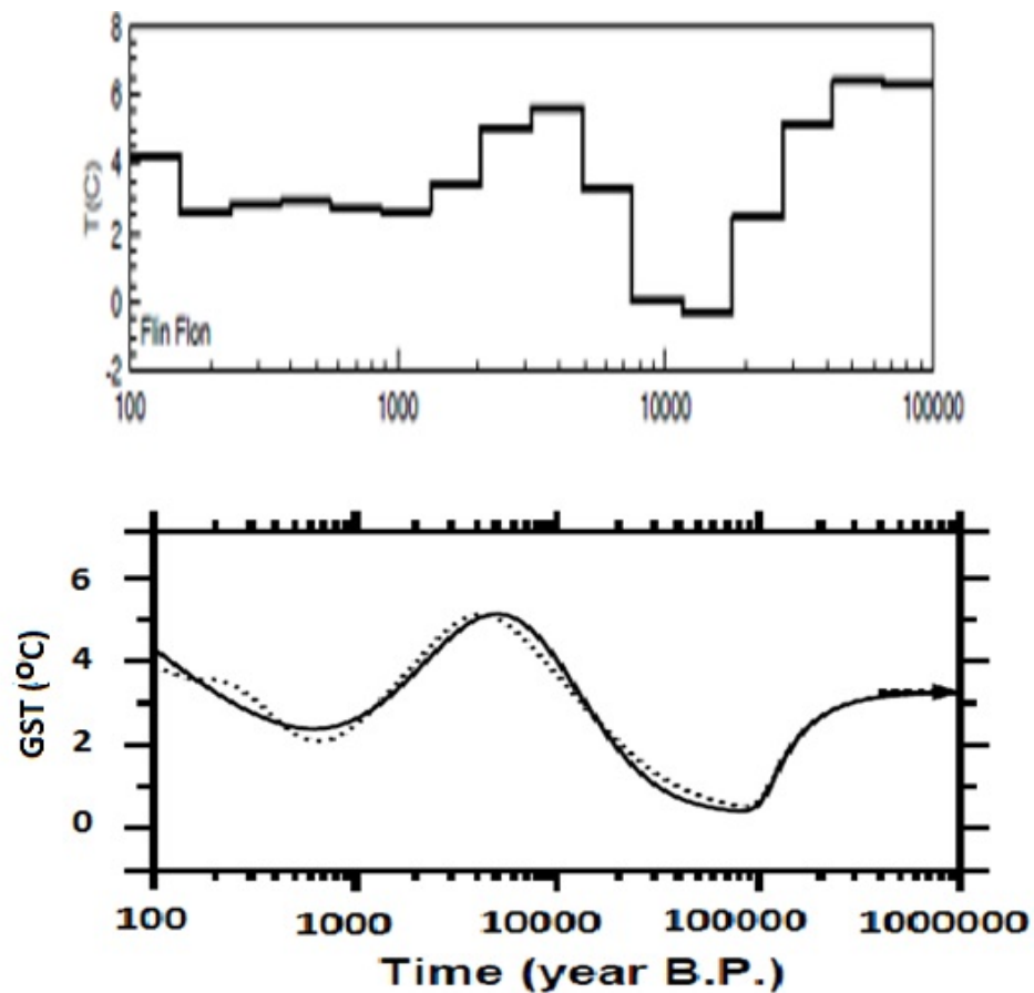
Fig. 2. Figure 2. Comparison of the two sets of results of inversions for GST history, using the same data set for Flin Flon (Manitoba). The upper panel illustrates the GST history reported in the discussion
