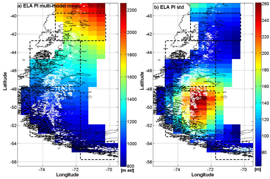
1 2 Figure 4. Spatial distribution of pre-industrial equilibrium line altitude (ELA) in South 3 America based on six PMIP2 simulations. (a) mean ELA (m asl) and (b) inter-model 4 variability of the ELA (one standard deviation). White lines correspond to actual glacier 5 extension according to the Randolph Glacier Inventory (RGI 3.2)
