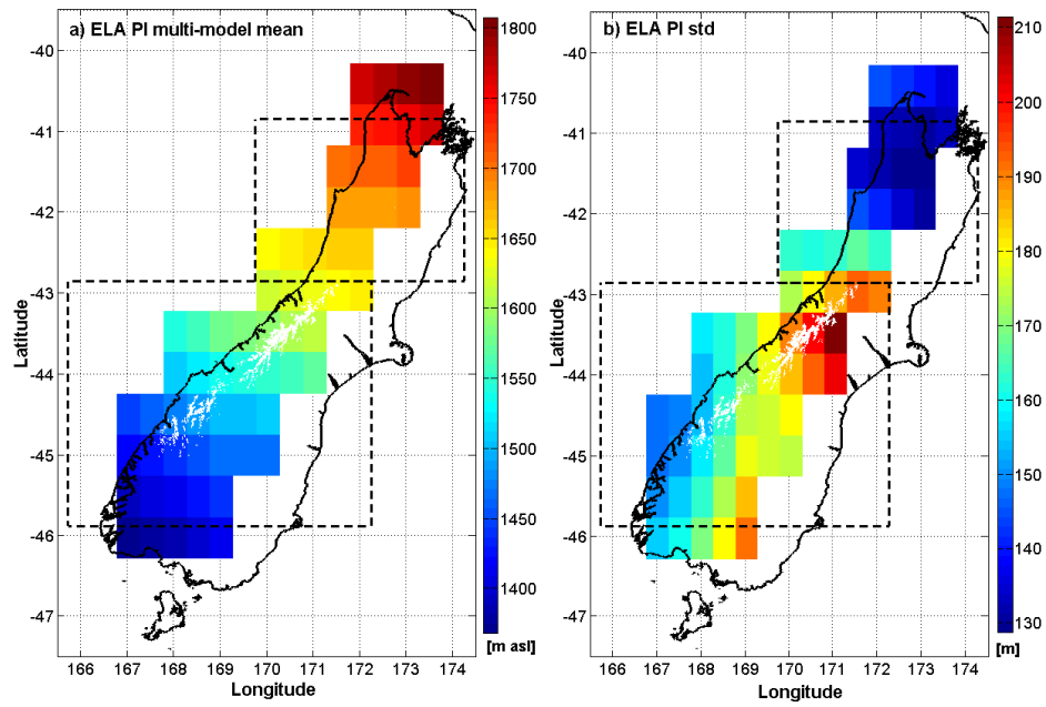
1 2 Figure 5. Spatial distribution of pre-industrial equilibrium line altitude (ELA) in Southern 3 Island of New Zealand based on six PMIP2 simulations. (a) Mean ELA (m asl) and (b) 4 inter-model variability of the ELA (one standard deviation). White lines correspond to 5 actual glacier extension according to the Randolph Glacier Inventory (RGI 3.2)
