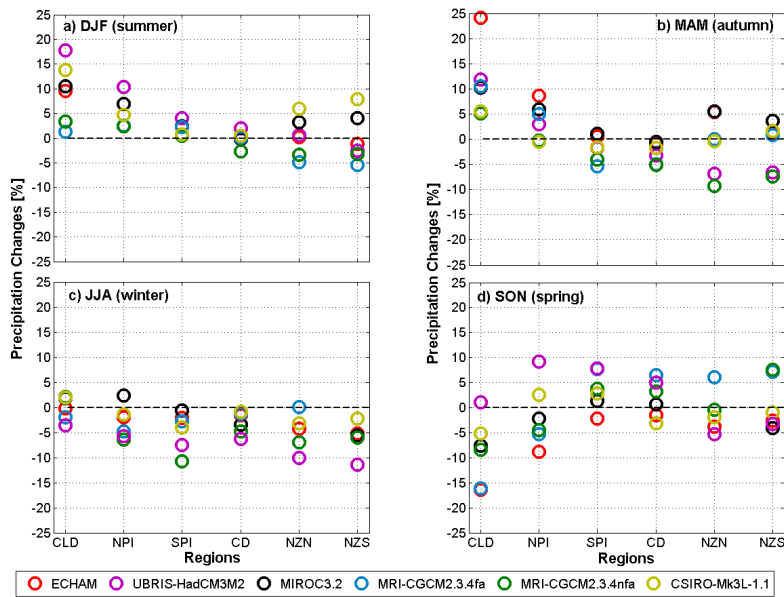
1 2 Figure 3. Precipitation differences: Mid-Holocene minus Preindustrial, over the 6 zones of 3 analysis. (a) DJF, (b) MAM, (c) JJA, (d) SON. Filled circles correspond to statistically 4 significant differences ( p \leq 0.05 ).
