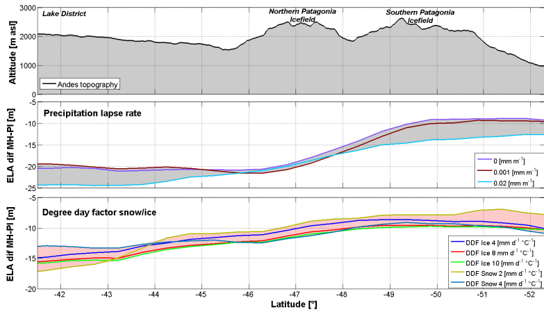
1 2 Figure 8. Sensitivity of ELA differences in Patagonian Andes to precipitation lapse rate and 3 degree day factor of snow and ice. a) Latitudinal topography profile of Patagonia (SRTM 1 4 km) b) ELA differences sensitivity to precipitation lapse rate and c) ELA differences 5 sensitivity to degree day factor of snow and ice. Gray and pink areas in b) and c) represent 6 the range in ELA differences between MH and PI.
