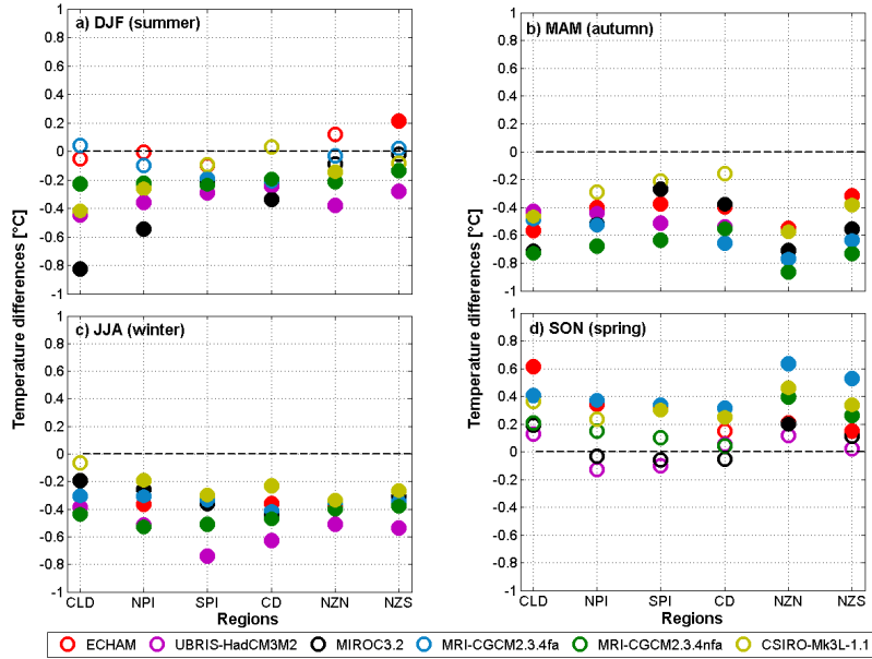
7 8 Figure 2. Temperature differences: Mid-Holocene minus Preindustrial, over the 6 zones of 9 analysis. (a) DJF, (b) MAM, (c) JJA, (d) SON. Filled circles correspond to statistically 10 significant differences ( p < 0.05 ).
