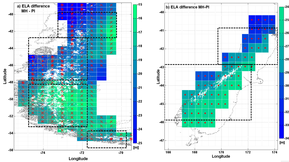
1 2 Figure 6. Mid-Holocene minus pre-industrial equilibrium line altitude differences. Points 3 indicate that the six models have a negative sign in the differences; asterisks indicate that 4 five models have a negative sign and crosses indicate that four models have a negative sign. 5 White lines indicate actual glacier outlines (Randolph Glacier Inventory 3.2). a) Patagonia, 6 b) New Zealand.
