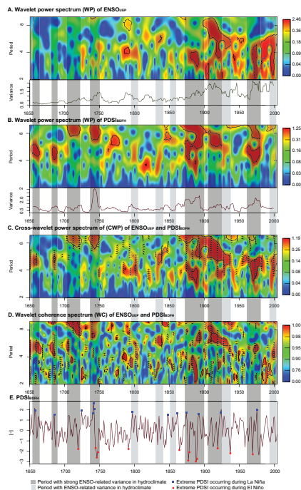
Figure 5. Wavelet analysis of the ENSO and PDSI BDFH over the period 1650–2004. Wavelet power spectrum of (a) ENSO UEP and (b) PDSI BDFH , (c) cross-wavelet power spectrum and (d) wavelet coherence spectrum of ENSO UEP and PDSI BDFH , and (e) time series of PDSI BDFH . Tiles (a) and (b) also show total variances of time series calculated with a moving window of 21 years. Dark grey columns indicate periods with strong ENSO-related variance in hydroclimate and the light grey columns indicate periods with ENSO-related variance in the PDSI BDFH . Tile (e) also shows extreme PDSI values that occurred during ENSO events. Extreme values were defined from PDSI data as 5th and 95th percentiles.
