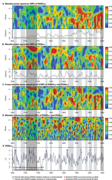
Figure 6. Wavelet analysis of the ENSO and PDSI_{MCC} over the period 1650–2004. Wavelet power spectrum of (a) ENSO_{UEP} and (b) PDSI_{MCC} , (c) cross-wavelet power spectrum and (d) wavelet coherence spectrum of ENSO_{UEP} and PDSI_{MCC} , and (e) time series of PDSI_{MCC} . Tiles (a) and (b) show also total variances of time series calculated with moving window of 21 years. Dark grey columns indicate periods with strong ENSO-related variance in hydroclimate and the light grey columns indicate periods with ENSO-related variance in the PDSI_{MCC} . Tile (e) also shows extreme PDSI values that occurred during ENSO events. Extreme values were defined from PDSI data as 5th and 95th percentiles.
