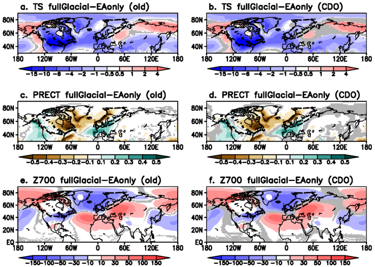
Fig 1. LGM changes (fullGlacial-EAonly) of the summer (JJA) temperature (a,b), annual precipitation (c,d) and JJA 700 hPa geopotential height anomaly (e,f). Only statistically significant changes (based on a Student's t-test at the 95% confidence level) are shown (non-significant values are depicted as gray shading). The left panels (a,c,e) show the statistically significant areas based on the erroneous calculations in the previous manuscript version, and the right panels (b,d,f) with the new corrected calculation using CDO.
