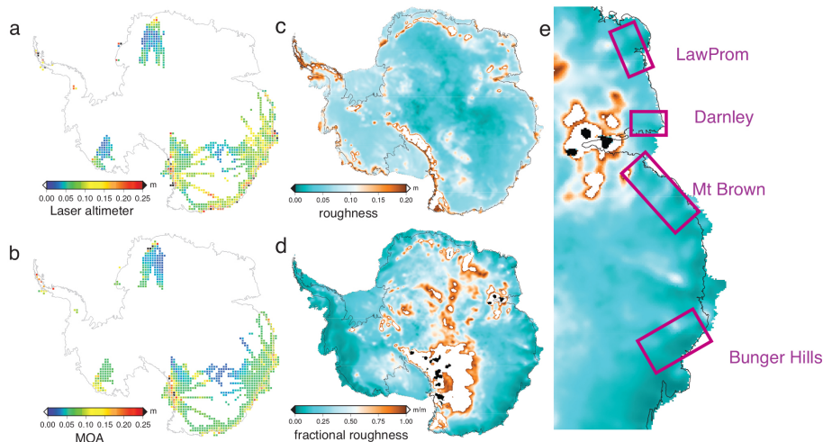
Figure 2. MODIS based surface roughness estimates. Panel (a) shows the calculated average surface roughness in each 50 km × 50 km grid, from Operation IceBridge, ICECAP and other University of Texas at Austin Institute of Geophysics Level 2 Geolocated nadir laser altimetry flight-line data (Blankenship et al., 2012; Young et al., 2015). Panel (b) shows the resultant estimate of surface roughness from MODIS Mosaic of Antarctica (MOA) imagery, by calibrating with the averaged surface altimetry calculated in panel (a) (see Method Sect. 3.3.2). Panel (c) shows the estimated (modelled) surface roughness for Antarctica using the laser altimetry-calibrated MOA imagery, while panel (d) shows estimated surface roughness as a fraction of estimated annual snowfall accumulation rate from RACMO2.1. In this instance, blue regions (low fractional roughness) indicate regions with minimal surface re-working as a fraction of snowfall accumulation rate, and hence potential high resolution ice coring sites. Panel (e) is the enlarged coastal East Antarctic section of the fractional roughness (panel d).
