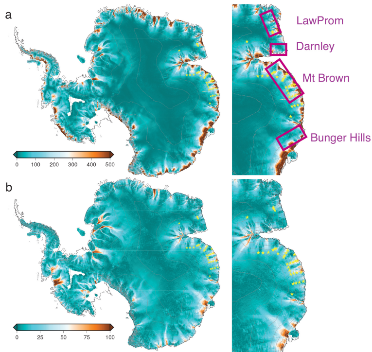
Figure 3. (a) Elevation change (m) and (b) ice advection (km) over 1000 years, calculated using a modified version of the Lagrangian streamline tracing of Roberts et al. (2011), with ice velocities from the MEASUREs dataset (Rignot et al., 2011). Blue areas show comparatively little elevation change and/or advection over 1000 years. The right hand panels are the enlarged coastal East Antarctic section of each panel. Stars indicate historical ice core locations for short records.
