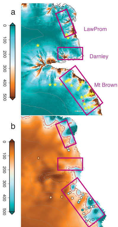
Figure 5. Further enlargement of (a) 3b (elevation change in metres), with the existing Mt. Brown South ice core record identified (fuchsia dot) and (b) Fig. 1b (annual snowfall accumulation with < 250 \text{ mm yr}^{-1} IE shown as solid red line).
