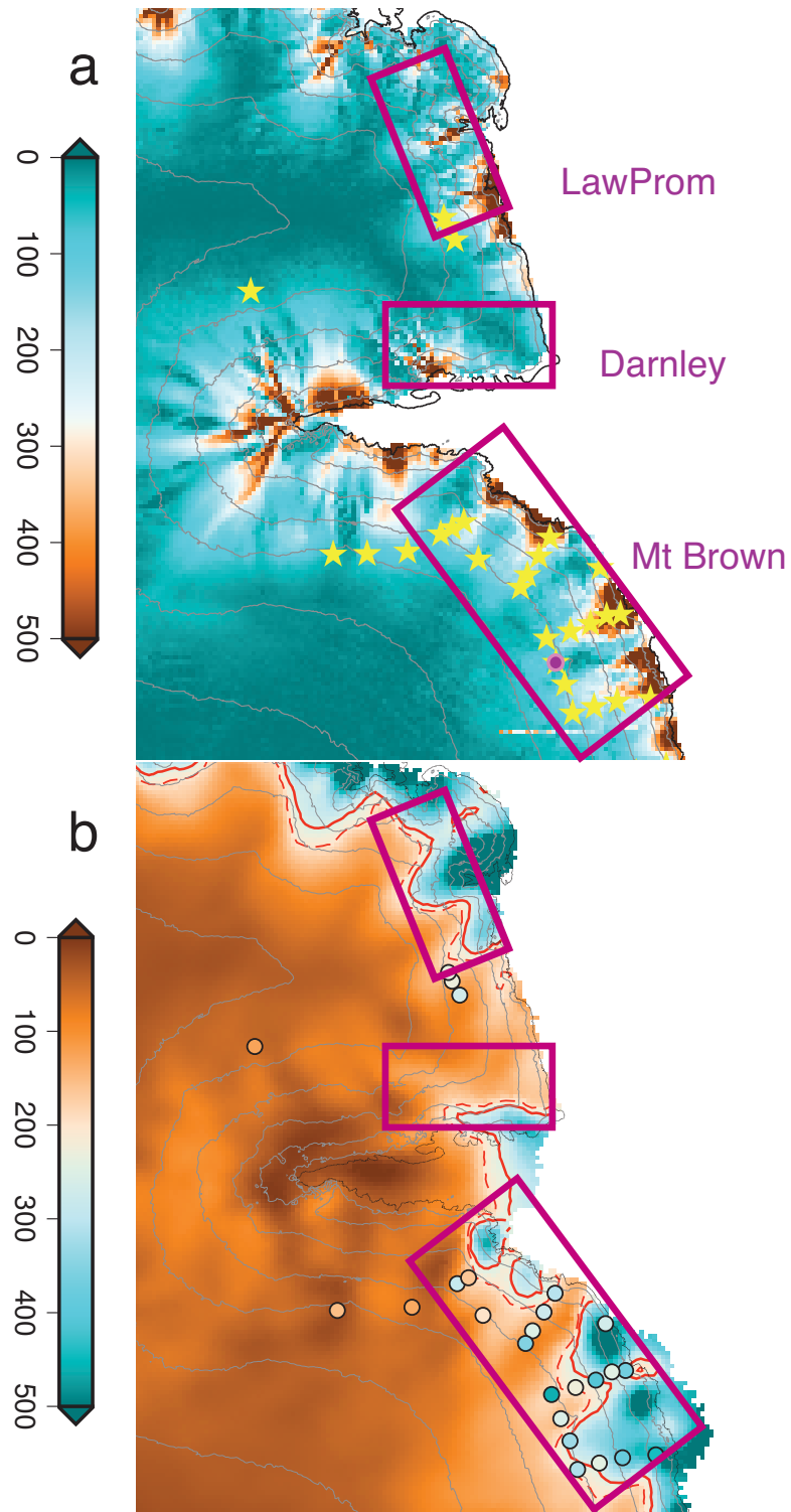
Figure 5. Panel (a) shows a further enlargement of Figure 3b (elevation change in metres), with the existing Mt. Brown South ice core record identified (fuchsia dot), while panel (b) shows a further enlargement of Figure 1b (annual snowfall accumulation with <250 \text{ mm y}^{-1} IE and <200 \text{ mm y}^{-1} IE shown as solid red and dashed red lines respectively).
