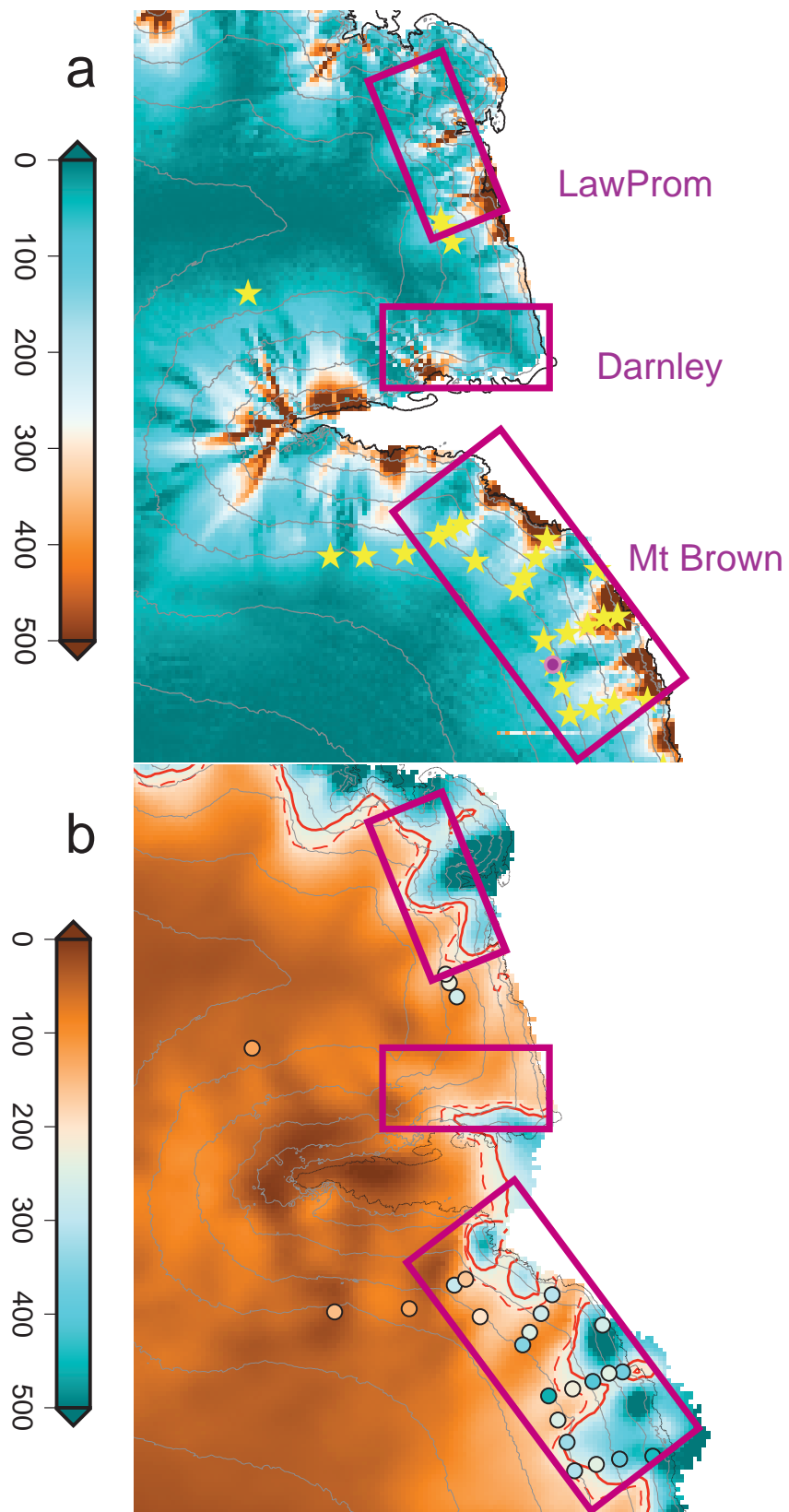
Figure 5. Further enlargement of (a) 3b (elevation change in metres), with the existing Mt. Brown South ice core record identified (fuchsia dot) and (b) Fig. 1b (annual snowfall accumulation with <250 \text{ mm y}^{-1} IE shown as solid red line).
