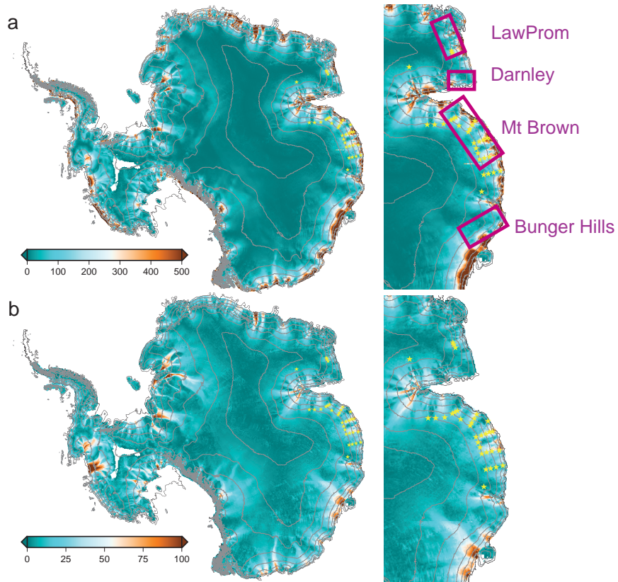
Figure 3. (a) Elevation change (metres) and (b) ice advection (kilometres) over 1000 years, calculated using a modified version of the Lagrangian streamline tracing of Roberts et al. (2011), with ice velocities from the MEASUREs dataset (Rignot et al., 2011). Blue areas show comparatively little elevation change and/or advection over 1000 years. The right hand panels are the enlarged coastal East Antarctic section of each panel. Stars indicate historical ice core locations for short records.
