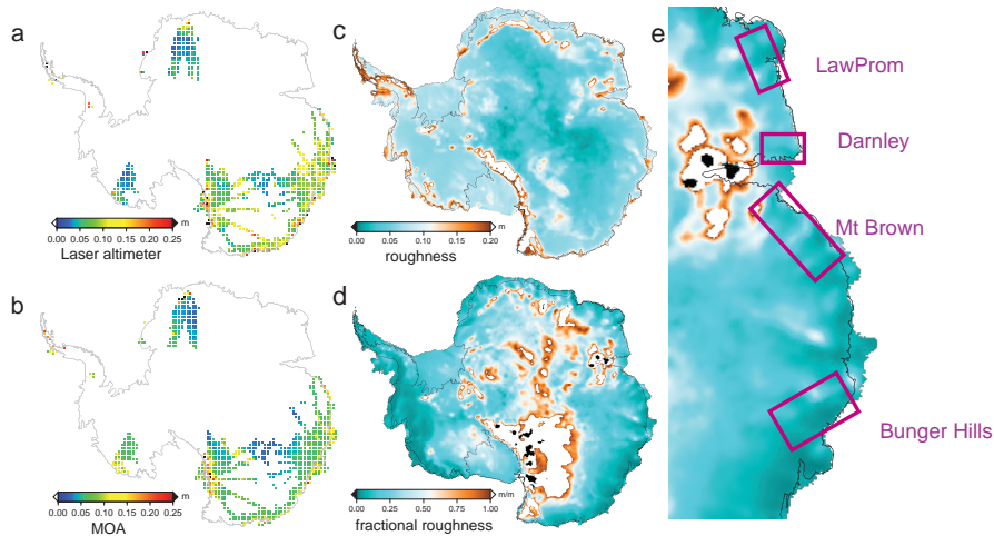
Figure 2. MODIS based surface roughness estimates. Panel (a) shows the calculated average surface roughness in each 50 \times 50 \text{ km}^2 grid, from Operation IceBridge, ICECAP and other University of Texas at Austin Institute of Geophysics Level 2 Geolocated nadir laser altimetry flight-line data (Blankenship et al., 2012; Young et al., 2015). Panel (b) shows the resultant estimate of surface roughness from MODIS Mosaic of Antarctica (MOA) imagery, by calibrating with the averaged surface altimetry calculated in panel (a) (see Method Section 3.3.2). Panel (c) shows the estimated (modelled) surface roughness for Antarctica using the laser altimetry-calibrated MOA imagery, while panel (d) shows estimated surface roughness as a fraction of estimated annual snowfall accumulation rate from RACMO2.1. In this instance, blue regions (low fractional roughness) indicate regions with minimal surface re-working as a fraction of snowfall accumulation rate, and hence potential high resolution ice coring sites. Panel (e) is the enlarged coastal East Antarctic section of the fractional roughness (panel d).
