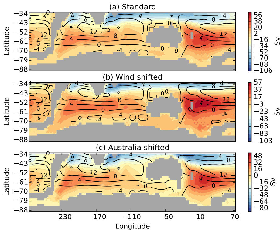
Figure 3. Ocean horizontal streamfunction (Sverdrup, 1 Sv is 10^6 \text{ m}^3 \text{ s}^{-1} ), with the zonal wind stress ( 10^2 \text{ Pa} ) overlaid. The Drake Passage is closed for (a) the standard simulation, (b) the Southern Hemisphere westerlies shifted north and (c) Australia and part of the Antarctic coast shifted north.
