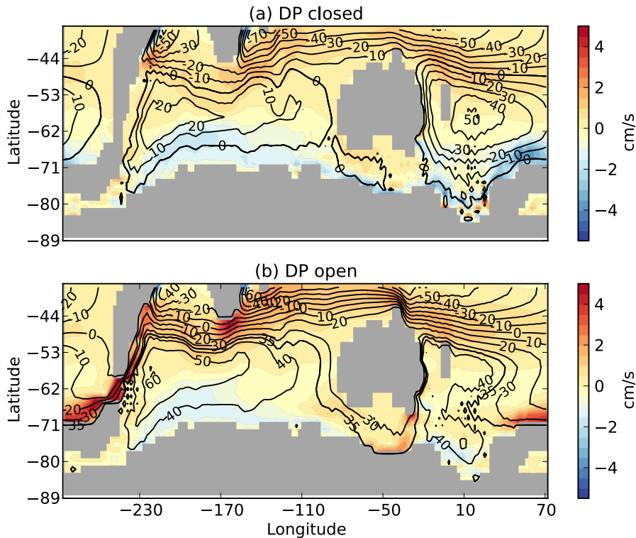
Figure 4. Annual and vertical average of zonal velocity ( \text{cm s}^{-1} , positive values indicate eastward flow) with ocean horizontal streamfunction (Sverdrup, 1 \text{ Sv} is 10^6 \text{ m}^3 \text{ s}^{-1} ) overlaid. The Tasman Gateway is open, with (a) the Drake Passage (DP) closed and (b) the DP open (shallow at around 350 m depth). Contour intervals have been adjusted in (a) to elucidate the flow through the TG.
