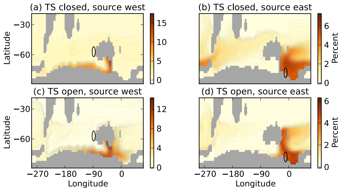
Figure 6. As Fig. 5, but for Drake Passage open. When the Tasman Gateway (TG) is open, dinoflagellates released to the west of Australia enter the Australo-Antarctic Gulf and flow into the Ross Sea through the TG (c) . Species released near the Ross Sea may enter the gulf along the Antarctic coast (d) .
