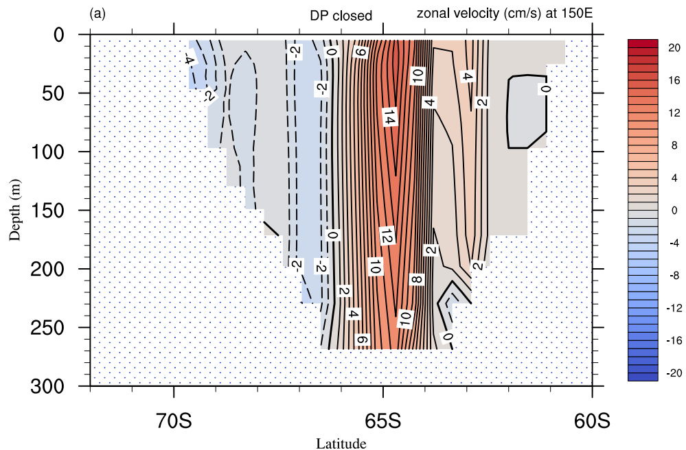
Figure 9. Meridional section of zonal velocity u ( \text{cm s}^{-1} ) inside the Tasman Gateway for the late Eocene POP simulation.
