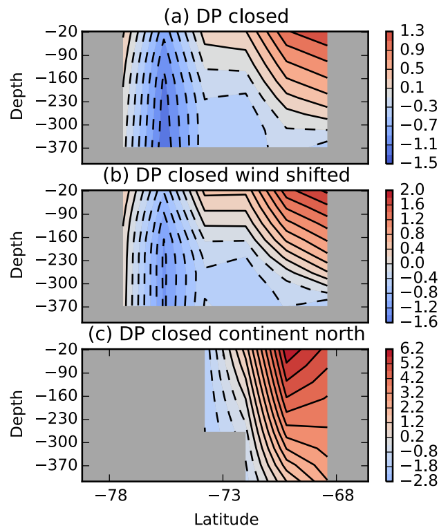
Figure 1. Meridional section of zonal velocity u ( \text{cm s}^{-1} ) inside the Tasman Gateway with Drake Passage closed, for (a) the standard simulation, (b) the Southern Hemisphere westerlies shifted 6 degrees northward, and (c) Australia and the Antarctic margin in a more northward position. All locations are well south of the latitudes of zero wind stress curl.
