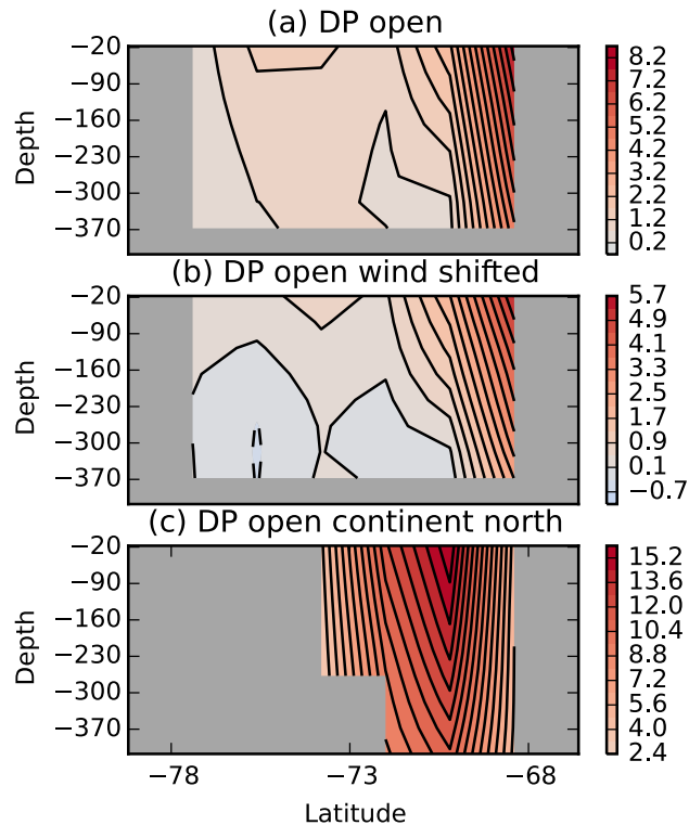
Figure 2. Meridional section of zonal velocity u ( \text{cm s}^{-1} ) inside the Tasman Gateway with Drake Passage open, for (a) the standard simulation, (b) the Southern Hemisphere westerlies shifted 6 degrees northward, and (c) Australia and the Antarctic margin in a more northward position. All locations are well south of the latitudes of zero wind stress curl.
