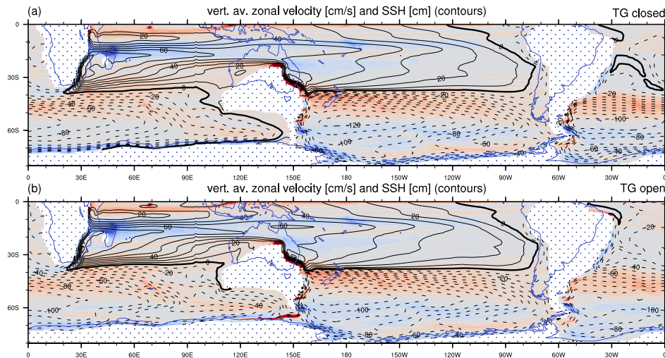
Figure 8. Annual and vertical average zonal velocity ( \text{cm s}^{-1} , positive values indicate eastward flow) with contours of sea surface height (SSH in cm) overlaid for the late Eocene simulation using a different ocean model (POP) with the Tasman Gateway (TG) closed (a) and open (b) . The Drake Passage is shallower than 35 m in these simulations and can be considered closed.
