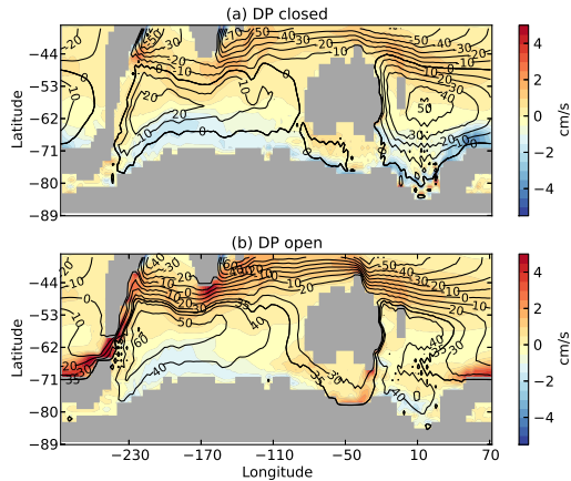
Figure 4. Annual and vertical average of zonal velocity ( cm/s , positive values indicate eastward flow) with ocean horizontal streamfunction (Sverdrup, 1 Sv is 10^6 m^3/s ) overlaid. The Tasman Gateway is open, with a) the Drake Passage (DP) closed and b) the DP open (shallow at around 350m depth). Contour intervals have been adjusted in (a) to elucidate the flow through the TG.
