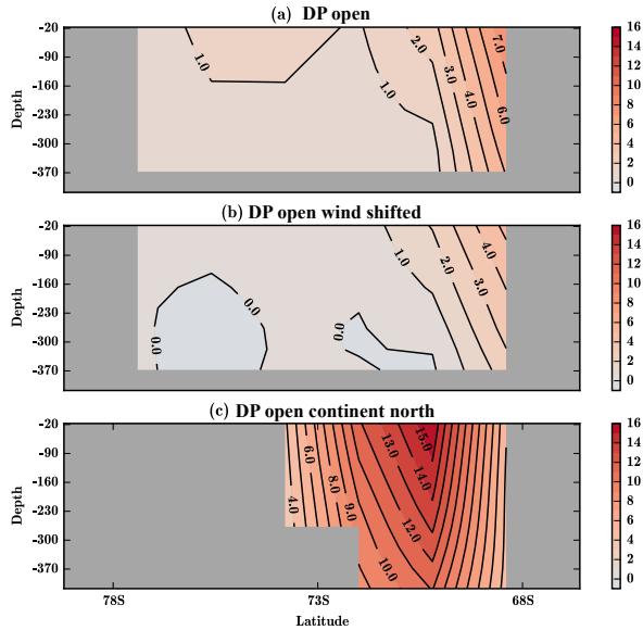
Figure 2. Meridional section of zonal velocity u ( cm/s ) inside the Tasman Gateway with Drake Passage open, for (a) the standard simulation, (b) the Southern Hemisphere westerlies shifted 6 degrees northward, and (c) Australia and the Antarctic margin in a more northward position. All locations are well south of the latitudes of zero wind stress curl.
