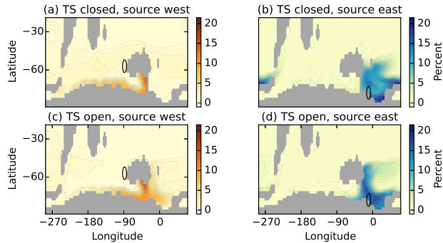
Figure 6. As figure 5, but for Drake Passage open. When the Tasman Gateway (TG) is open, dinoflagellates released to the west of Australia enter the Australo-Antarctic Gulf and flow into the Ross Sea through the TG (c). Species released near the Ross Sea may enter the gulf along the Antarctic coast (d). We examine a snapshot taken 5 years after tracer release.
