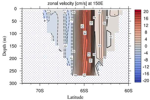
Figure 10. Meridional section of zonal velocity u (cm/s) inside the Tasman Gateway for the late Eocene POP simulation.
