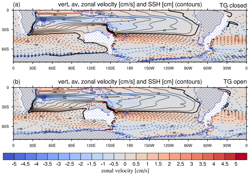
Figure 9. Annual and vertical average zonal velocity ( cm/s , positive values indicate eastward flow) with contours of sea surface height (SSH in cm ) overlaid for the late Eocene simulation using a different ocean model (POP) with the Tasman Gateway (TG) closed (a) and open (b). The Drake Passage is shallower than 35 m in these simulations and can be considered closed.
