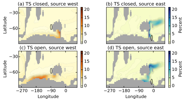
Figure 5. Dispersal of passive tracer representing dinoflagellates for Drake Passage closed for the Tasman Gateway (TG) closed, originating west (a) and east (b) of Australia, and for TG open, originating west (c) and east (d) of Australia. Circles indicate the release sites. When the TG is open, dinoflagellates released to the west of Australia enter the Australo-Antarctic Gulf predominantly along the Australian coast, but remain west of the TG and do not enter the Ross Sea (c). In contrast, species released near the Ross Sea may enter the gulf via a westward flow along the Antarctic coast (d). Concentrations are in percentages, where the initial localised concentration upon release was 100 percent. We examine a snapshot taken 5 years after tracer release.
