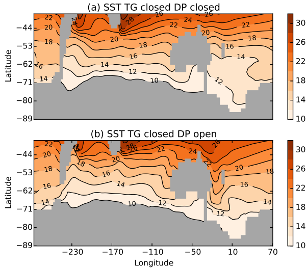
Figure 8. Sea Surface Temperature for a) Drake Passage (DP) closed and b) DP open.
