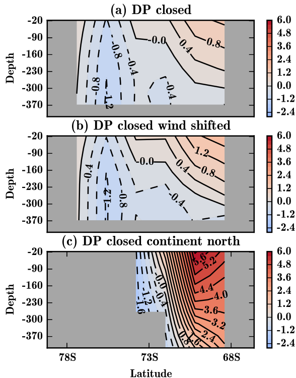
Figure 1. Meridional section of zonal velocity u ( cm/s ) inside the Tasman Gateway with Drake Passage closed. for (a) the standard simulation, (b) the Southern Hemisphere westerlies shifted 6 degrees northward, and (c) Australia and the Antarctic margin in a more northward position. All locations are well south of the latitudes of zero wind stress curl. Positive values indicate eastward flow, negative values indicate westward flow.
