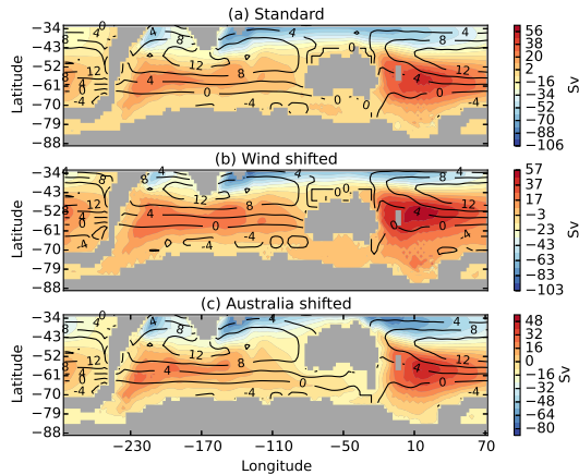
Figure 3. Ocean horizontal streamfunction (Sverdrup, 1 \text{ Sv} is 10^6 \text{ m}^3/\text{s} ), with the zonal wind stress ( 10^2 \text{ Pa} ) overlaid. The Drake Passage is closed for a) the standard simulation, b) the southern hemisphere westerlies shifted north and c) Australia and part of the Antarctic coast shifted north.
