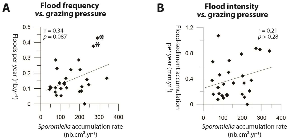
Fig. S3. Representation and correlation coefficients ( r ) of relations between (A) Sporormiella accumulation rates (nb.cm 2 .yr -1 ) and floods frequency (nb.yr -1 ), and between (B) Sporormiella accumulation rates (nb. cm 2 yr -1 ) and flood-sediment accumulation (mm.years -1 ). The stars identified two samples, dated from 1734 to 1760 AD, with both high grazing pressure and high flood frequency. Levels of significance ( p values) were determined using a Spearman-test.
