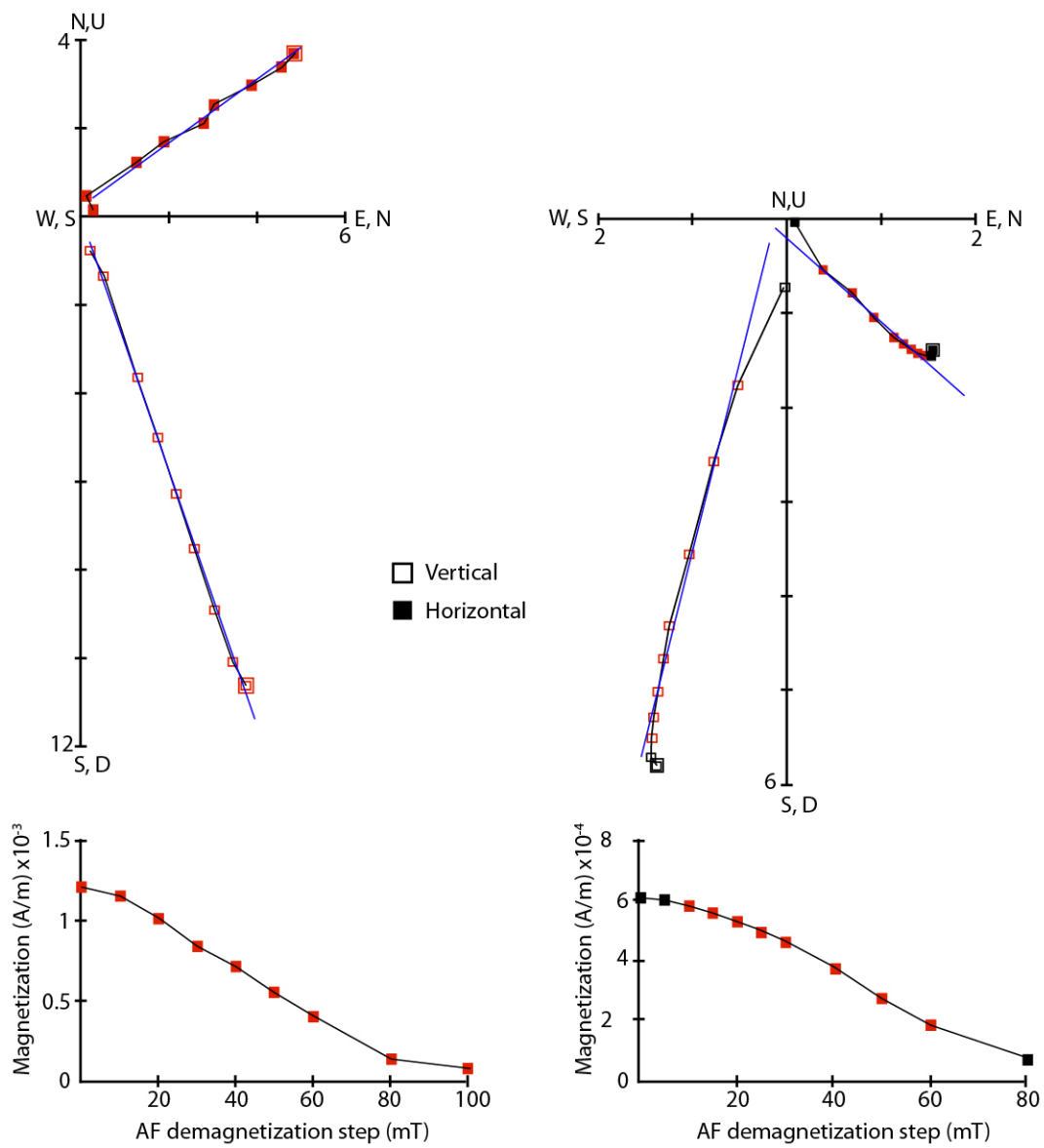
Fig. S2. Example of stepwise alternating field demagnetization of NRM (orthogonal vector projections and intensity curves) for representative samples. Solid (open) symbols are horizontal (vertical) plane projections.
