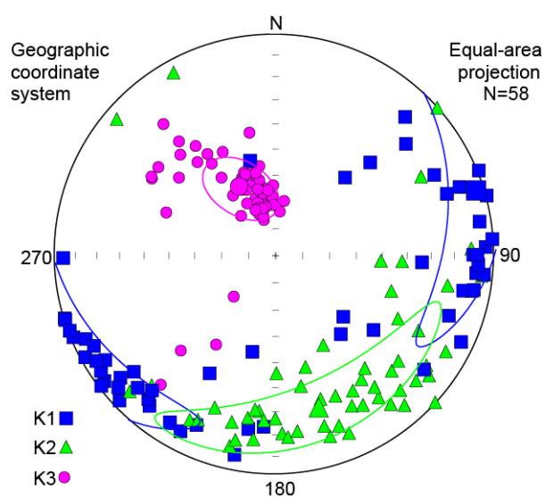
Fig. S1. Results of Anisotropy of Magnetic Susceptibility for core FOR13P4: stereo plot of the main axes direction. Notice that the K3 is well grouped and close to the vertical except some points associated with MMITs.
