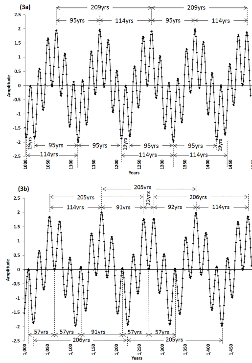
Figure 3. SdV and Gleissberg cycles. Combination of the RRA, Metonic and sunspot cycles reproduce the SdV and Gleissberg cycles; (a) Combined RRA and Metonic sinusoidal curves SdV (209 years) and Gleissberg (95 years); (b) Combined RRA and sunspot sinusoidal curves: SdV (205–206 years) and Gleissberg (91 years).
