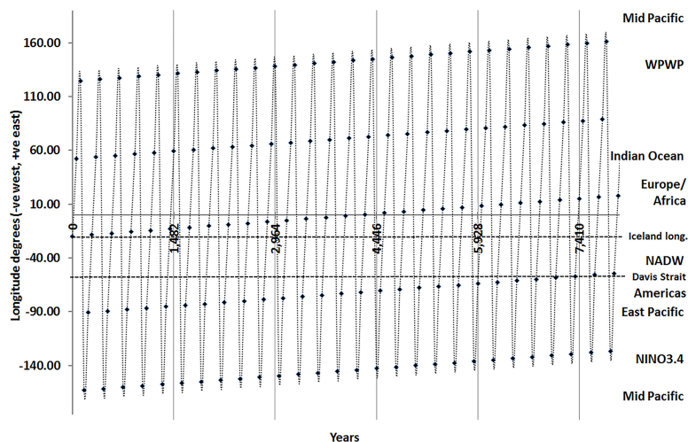
Figure 2. The 57 year Metonic-sunspot cycle in geographic context. Vertical axis represents geographic longitude and horizontal axis time in years, from an arbitrary start for 80 centuries. Time between points on the Metonic-sunspot curve is 57 years, and time between points at the same longitude is 285 years. The 1482 year Metonic-sunspot period (solid vertical lines) is close to the RRA cycle of 1479 years. The 285 year and 1482 year periodicities are harmonics of the 57 year cycle.
