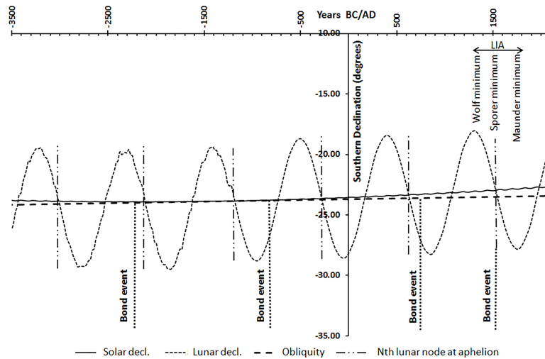
Figure 1. Solar and lunar declination interaction of the Metonic-perihelion cycle at 19 yr intervals. Bond IRD events occurred close to the lunar nodes at aphelion/perihelion. Total and annular solar eclipses occur at the juncture of these solar and lunar declinations. The relationship of these cycles to the ecliptic is shown through the dotted line associated with obliquity. Solar declinations form the solid sinusoidal curve, and lunar declinations the dashed sinusoidal curve; the dashed line is the ecliptic.
