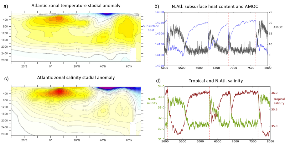
Figure 5. Thermohaline oscillations in the Unhosed simulation. a,c) Atlantic zonally-averaged temperature and salinity anomaly anomalies between weak AMOC state (years 7501-7600) state and strong AMOC state (years 7901-8000). Units in °C and PSU, respectively . b) Subsurface (500-2500m) heat content in the North Atlantic (>45°N in zettajoules (blue) Units and AMOC transport in ZettaJoulesSv (black). d) Sea surface salinity in the North Atlantic (>45°N) (black) and Tropical Atlantic (0:10 °N, 70:30 °W) (red) Units , in PSU. Red vertical dashed lines indicate onset of deep convection in the North Atlantic.
