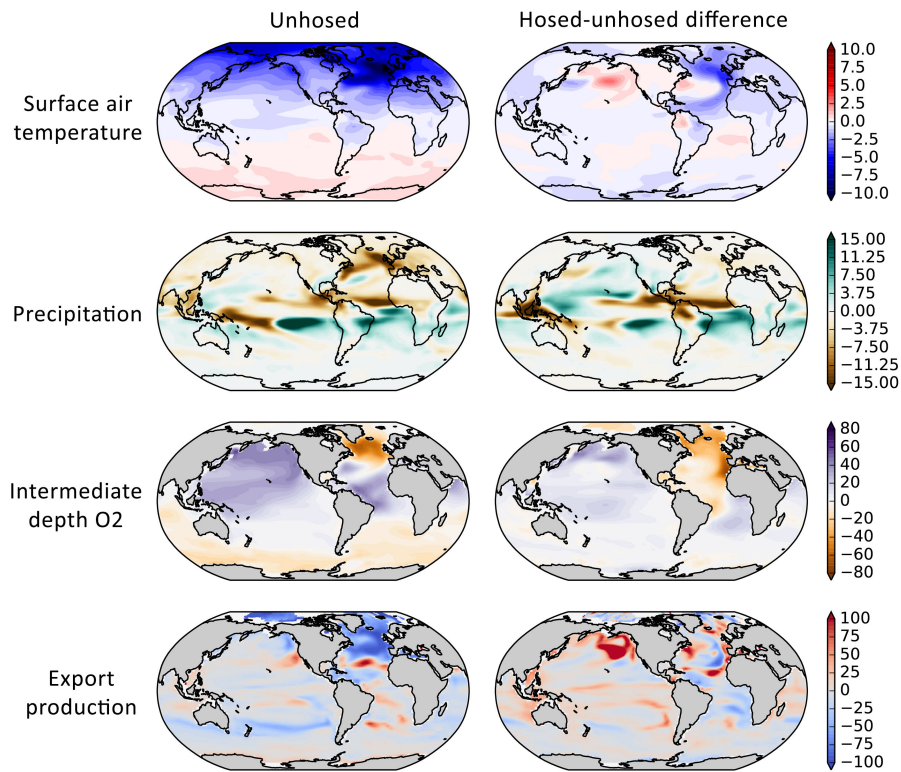
Figure 11. Impacts of hosing the Unhosed. Differences —Left column: differences between weak and strong AMOC states for the unhosed simulation as shown in figures 6,7,8 and 9. Right column: differences between the last century (model years 6151-6250) of the 800-year hosed-Unhosed stadial and the corresponding unhosed stadial. Scale and units are the same as in figures 6,7,8, and 9: temperature in °C, precipitation in 10^{-6} \text{ kg m}^{-2} \text{ s}^{-1} , oxygen concentration in in \mu\text{mol kg}^{-1} and export anomaly in %.
