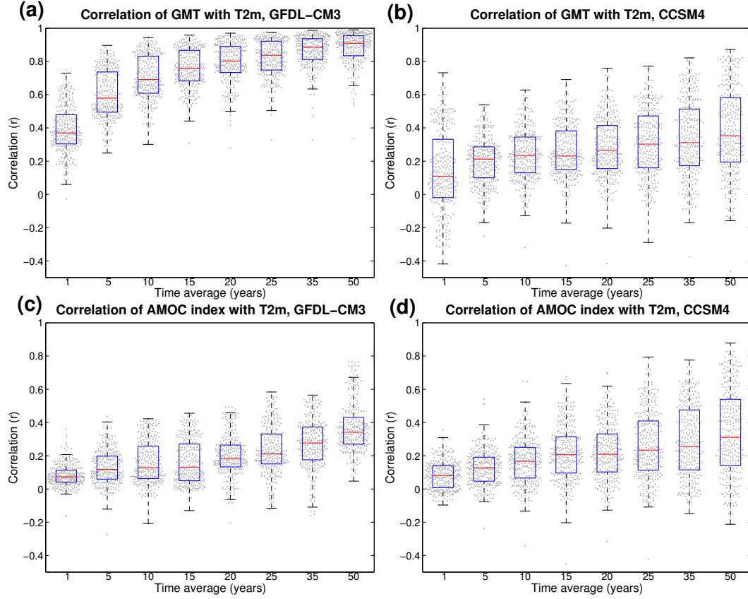
Figure 4. (a) and (b) show the distribution of correlation values between the global-mean 2-m air temperature (GMT) and the spatial -2-m air surface temperatures (T2m) at the proxy locations for GFDL-CM3 and CCSM4 at a range of time-averages. (c) and (d) show similar correlation distributions but for the correlation between the Atlantic meridional overturning circulation (AMOC) index and the spatial -2-m air surface temperatures at the proxy locations . The correlations are computed for each-spatial-proxy grid point -points at a given time-average, with the spatial-correlation-information distribution of these correlations shown in gray dots and also summarized with-by box plots ( outliers have been omitted for clarity ).
