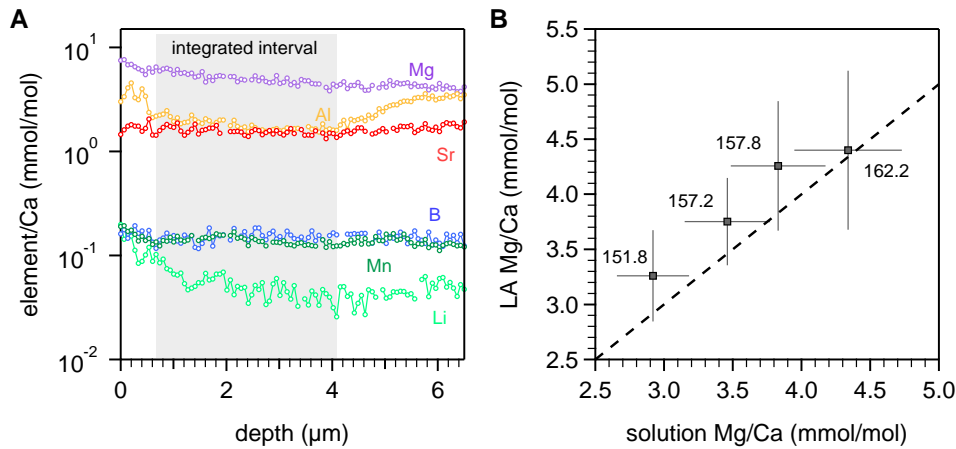
Figure 3. (a) An example laser ablation profile through a Turborotalia ampliapertura chamber. Sub-μm variations in element/Ca ratios are identifiable, enabling poorly preserved or contaminated areas of the test to be excluded from the calculation of mean values. Here, the inner and outer surfaces of the chamber are characterised by elevated Al/Ca, implying incomplete clay particle removal. (b) A comparison of laser-ablation and solution ICPMS Mg/Ca data from the same intervals at St. Stephens Quarry. Solution data from Wade et al. (2012). Labels show the depth intervals of these samples. Solution ICPMS error bars are the long-term precision (RSD), whereas laser-ablation error bars are 2SE of all analyses from each interval.
