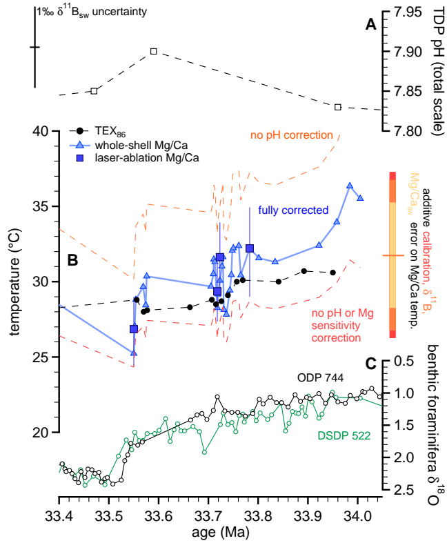
Figure 8. (a) EOT pH reconstruction from Pearson et al. (2009) based on Tanzania Drilling Project samples. The error bar is derived from an uncertainty in \delta^{11}\text{B}_{\text{sw}} of \pm 1\% . (b) Subtropical sea surface temperature from Mg/Ca and \text{TEX}_{86} . These absolute Mg/Ca temperatures are the first to be adjusted for both the pH effect on Mg incorporation and the nonlinear relationship between seawater-shell Mg/Ca and temperature. St. Stephens Quarry Mg/Ca data from both solution ICPMS Wade et al. (2012) and laser ablation (this study) are shown. The combined Mg/Ca error estimate is that due to uncertainty in the \text{Mg}/\text{Ca}_{\text{sw}} ratio ( \pm 0.5 \text{ mol mol}^{-1} ), \delta^{11}\text{B}_{\text{sw}} and in the calibration regressions of Evans et al. (2016). The corrected Mg/Ca data imply 6^\circ\text{C} of precursor cooling at \sim 33.9 \text{ Ma} . (c) ODP Site 744 and DSDP Site 522 benthic foraminifera \delta^{18}\text{O} (Zachos et al., 1996). Note that the inter-interval Mg/Ca and \delta^{11}\text{B}_{\text{sw}} error (i.e. the error in relative changes) is far smaller than shown by the bars.
