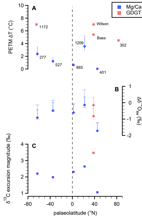
Figure 7. Compiled sea surface temperature and \delta^{18}O_{sw} peak PETM shifts relative to pre-CIE values. (a) GDGT and Mg/Ca-derived warming as a function of latitude. Mg/Ca estimates are adjusted for both pH and the sensitivity of the Mg/Ca-temperature relationship in PETM seawater (see text for details), and are the average of estimates derived from the two surface-dwelling foraminifera genera Morozovella and Acarinina . Labels refer to ODP/DSDP site numbers or locality names. (b) \Delta\delta^{18}O_{sw} reconstructions based on foraminifera \delta^{18}O coupled with either Mg/Ca or GDGT-derived sea surface temperature shifts. \delta^{18}O was adjusted for pH following Uchikawa and Zeebe (2010). Inner error bars are the uncertainty relating to the \delta^{18}O -pH slope (datapoints use the \delta^{18}O -pH slope of G. bulloides whilst the inner positive error bar shows where the data would lie if the slope of O. universa were to be used), outer error bars also include the uncertainty relating to the pH and sensitivity corrections applied to the Mg/Ca data. Data not specifically discussed in the main text are from Sluijs et al. (2006) and Sluijs et al. (2011). (c) The magnitude of the carbon isotope excursion at each site in Acarinina , with the exception of DSDP Site 401 ( Morozovella ).
