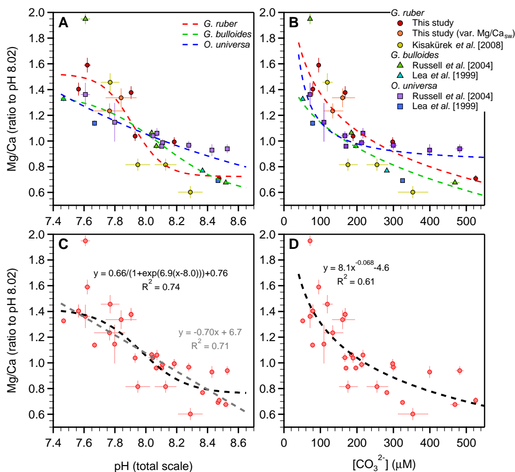
Figure 1. New and compiled planktic foraminifera Mg/Ca-carbonate chemistry data. Mg/Ca is shown as a ratio to that at pH 8.02 (~ 8.15 on the NBS scale) for each species. (a) Species-specific Mg/Ca variation with pH. (b) Mg/Ca variation with [\text{CO}_3^{2-}] . (c, d) show the same datasets with regressions calculated from all data combined. Both logistic and linear relationships are shown between Mg/Ca and pH.
