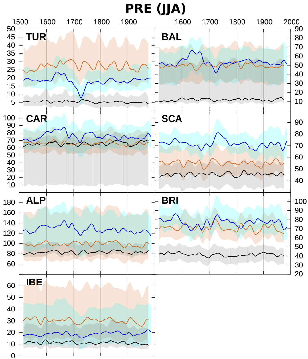
Figure 5. As Fig. 4 but for summer PRE.
