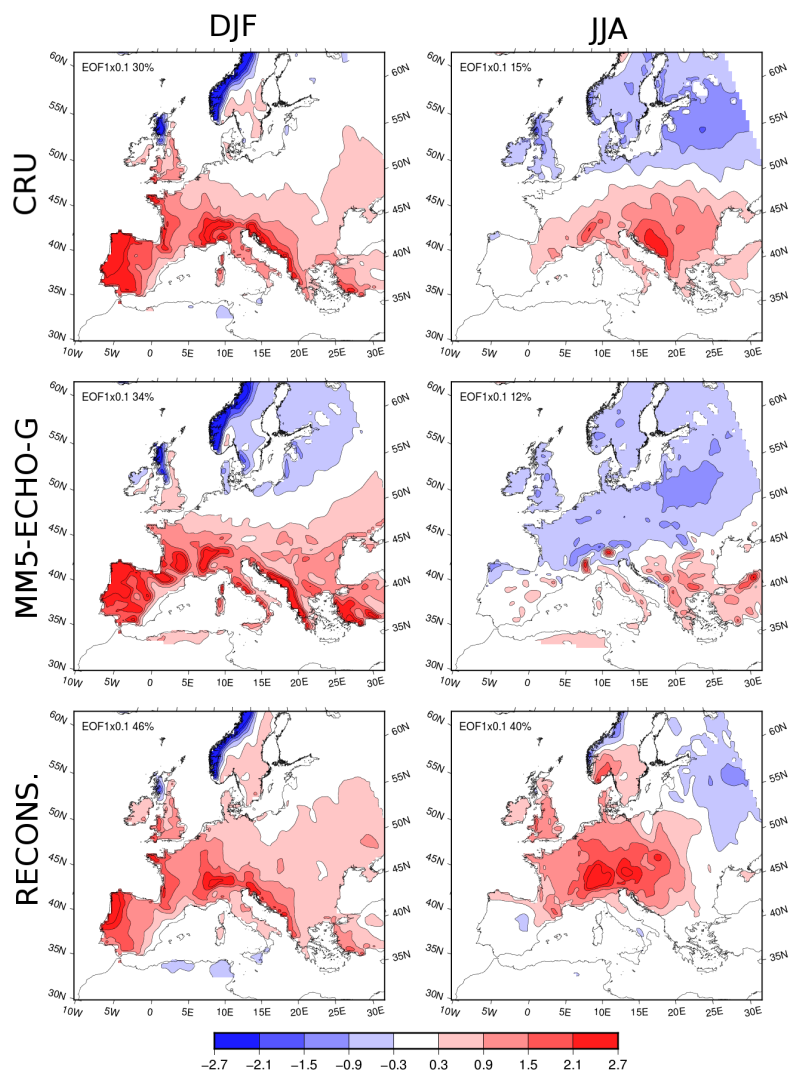
Figure 9. As Fig. 8 but for PRE. The units are mm/month.
