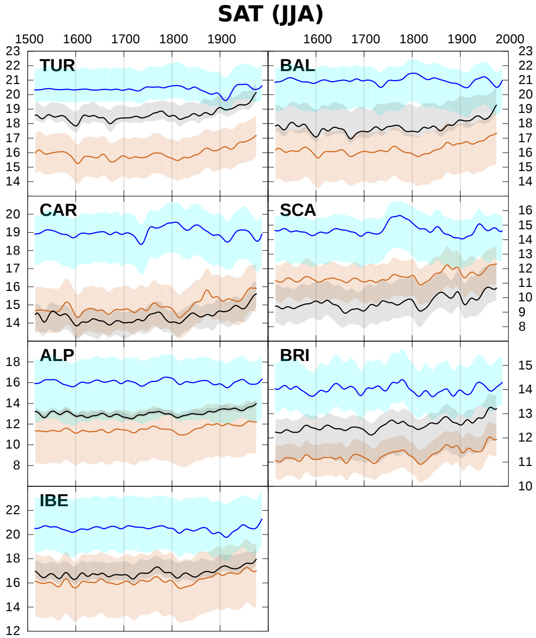
Figure 3. As Fig. 2 but for simulated summer SAT.
