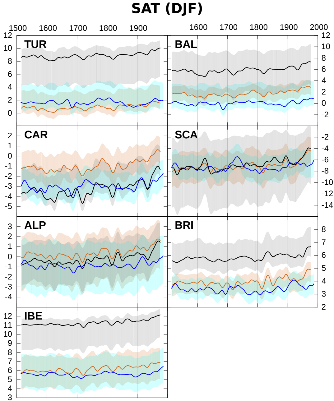
Figure 2. Temporal series of winter SAT in the seven areas indicated in Fig. 1 that exhibit added value in the MM5-ECHO-G simulation compared to the GCM alone according to Gómez-Navarro et al. (2013). The series corresponding to the three different data sets are shown with different colours: driving GCM (i.e. ECHO-G model alone, black), RCM (i.e. MM5-ECHO-G, orange) and gridded reconstruction (i.e. the Luterbacher et al. (2004) reconstruction, blue). Bold lines correspond to the median, whereas the light shading indicates the 25-75 interquartile range to illustrate heterogeneities within each region. After the calculation of the annual values, the series are smoothed through a Hamming window of 31 time steps to emphasise the low-frequency variability. Note the different scale in different panels.
