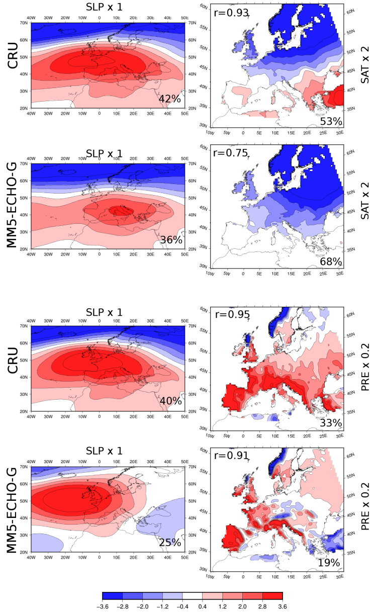
Figure 10. Canonical correlation pattern pairs of SLP and SAT (rows 1 and 2), and SLP and precipitation (rows 3 and 4) in winter. Each panel depicts the percentage of variance explained by each pattern and the canonical correlation associated with the pair. The results are calculated in the observational record (rows 1 and 3) and in the MM5-ECHO-G data set (rows 2 and 4) during the period 1901–1990. Note that the SLP has been obtained directly from the driving GCM, since the window of interest lies outside the RCM domain. As in Figs. 8 and 9, the patterns have been multiplied by a scaling factor that allows using the same color scale in every map. The SAT units are °C, SLP is shown in Pa, whereas precipitation units are mm/month.
