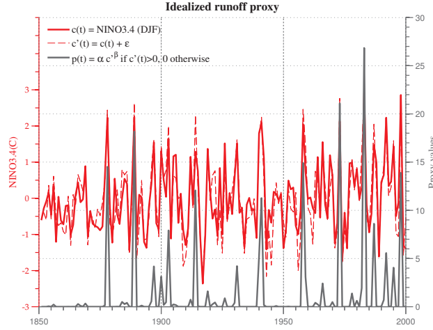
Figure 1. A nonlinear recorder of ENSO activity. Solid red: December-January-February average of the NINO3.4 index from the ERSSTv3 dataset (Smith et al., 2008), standardised to Z scores; dashed red: standardised NINO3.4 with additive \mathcal{N}(0, 0.25) noise; gray: the noisy NINO3.4 signal transformed according to Eq.(1), with \alpha = 1 and \beta = 3 .
