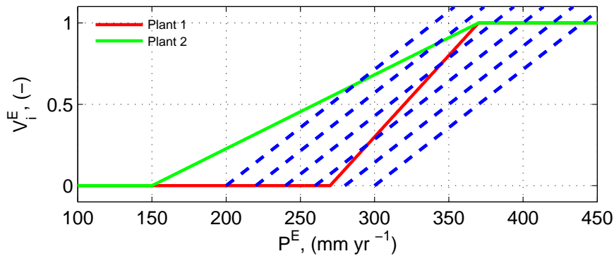
Figure 1. Vegetation–precipitation stability diagram ( V_i^E , P^E ) for two hypothetical plant types i = 1, 2 after Claussen et al. (2013). Full lines depict the equilibrium curves for vegetation cover V_i^E(P^E) for plant type 1 which is sensitive (red) and for plant type 2 which is resilient (green) to changes in precipitation. Dashed blue lines show hypothetical equilibrium precipitation curves P^E(V_i^E) for different time slices (4500, 4900, 5300, 5700, 6100, and 6500 years BP, from left to right). Intersections between the two types of curves indicate equilibrium coupled states which can be stable or unstable.
