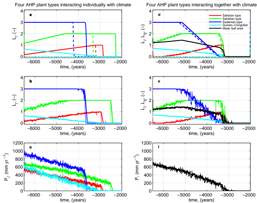
Figure 3. Transient dynamics of four African Humid Period (AHP) plant types interacting individually (a–c) and together (d–f) with climate. The effective leaf areas L_i and the corresponding precipitation amounts P_i are shown for the Saharan type (red), Sahelian type (green), Sudanian type (blue) and Guineo–Congolian type (light blue). Mean effective leaf area L_S and the corresponding precipitation P are calculated with the niche approach (black) (see Eq. 9). Simulations without background noise (a, e) include forward simulations (solid lines) and simulations backward in time (dashed lines). Simulations with background noise are depicted in (b, e) for L_i and L_S , and for precipitation P in (c, f). Thin lines show annual mean values and thick lines show a 100 year running mean.
