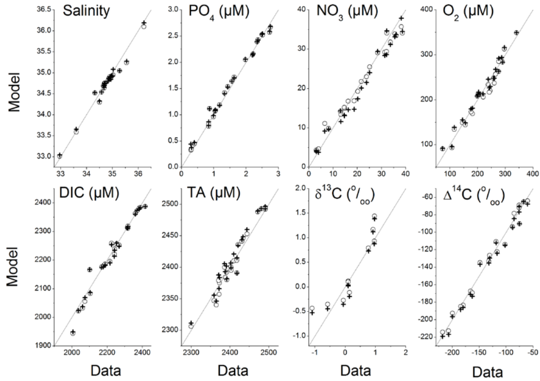
Fig. A1. Tracer concentrations in ocean boxes: Model versus data. Open circles indicate concentrations applied as initial values at 130 ka (Tab. A1 and A2). Crosses are concentrations obtained at the end of simulation STD at 0 ka after the completion of a full glacial cycle. Lines indicate the 1:1 relationship, e.g. the best fit to the data. \delta^{13}\text{C} data at <2000 m water depth are excluded from the model-data comparison since they are affected by anthropogenic \text{CO}_2 .
