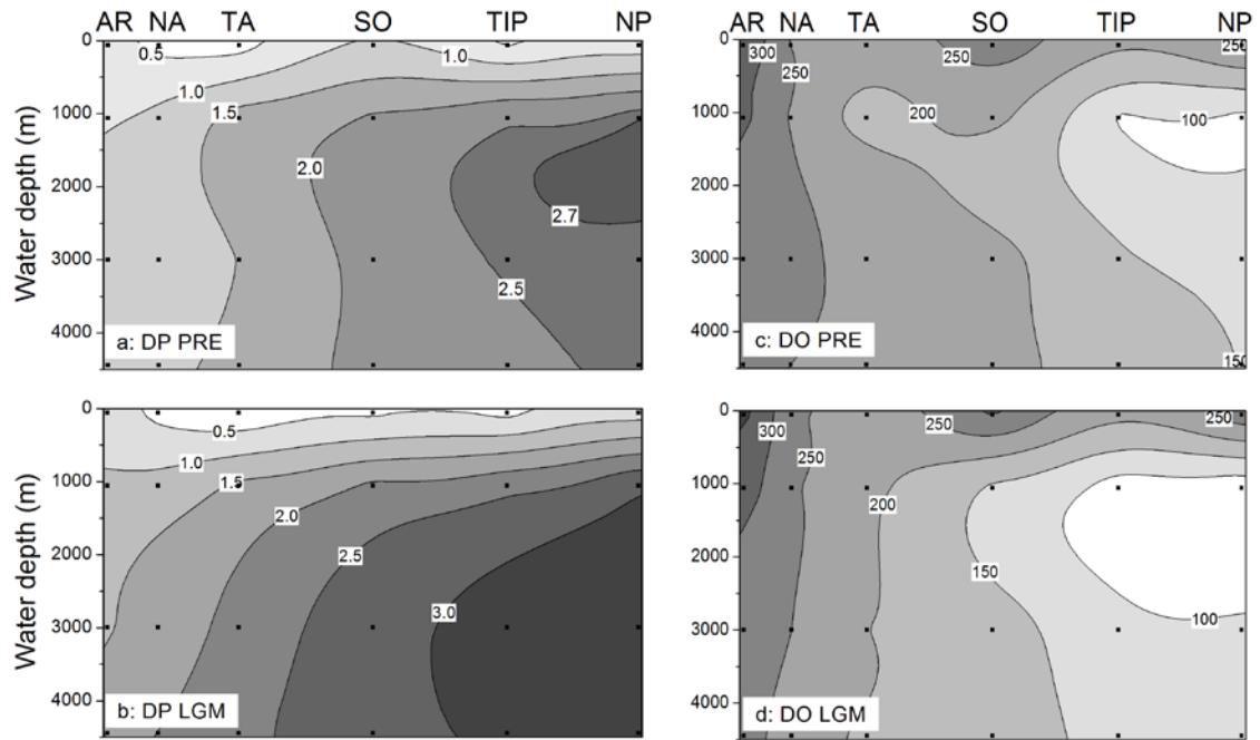
Figure 8. Concentrations (in \mu\text{M} ) of dissolved phosphorus (DP) and oxygen (DO) in the pre-anthropogenic modern ocean (PRE, model results for 0 ka, a: DP, c: DO) and during the LGM (model results for 21 ka, b: DP, d: DO, Tab. C4). The contour plots shown here and in Figures 9 and 11 are based on concentrations calculated in simulation STD for each of the 24 ocean boxes (indicated as grid points).
