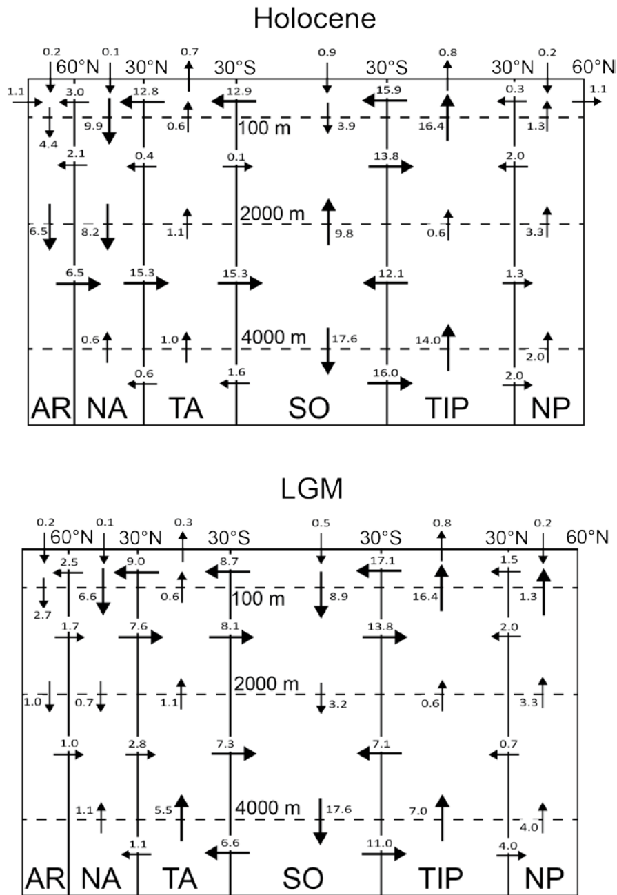
Figure 2. Set-up of the box model: The global ocean is separated into 24 boxes representing surface (0 – 100 m), intermediate (100 - 2000 m), deep (2000 – 4000 m), and bottom (>4000 m) waters in the Arctic (AR), North Atlantic (NA), Tropical Atlantic (TA), Southern Ocean (SO), Tropical Indo-Pacific (TIP), and North Pacific (NP) . Arrows with numbers indicate net water fluxes between boxes in Sv; major fluxes (>5 Sv) are represented by large arrows, minor fluxes (<5 Sv) by small arrows. Arrows crossing the top boundary of the surface water boxes (seawater-atmosphere interface) indicate net freshwater fluxes (precipitation + river water fluxes - evaporation). The upper panel shows the circulation field applied for the modern ocean and the previous interglacial, the lower panel shows the circulation applied over the LGM.
