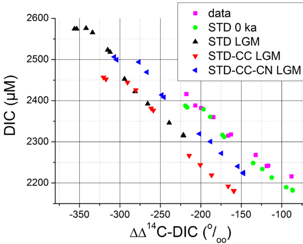
Figure 13. DIC versus difference between radiocarbon in seawater DIC and atmospheric CO 2 ( \Delta\Delta^{14}\text{C-DIC} ) at >2000 m water depth. Data are mean values for deep water and bottom water boxes derived from water column measurements. Model results are shown for the standard case (STD), for constant circulation (STD-CC), and constant values for circulation and nutrient utilization (STD-CC-CN). LGM refers to model results at 21 kyr BP.
