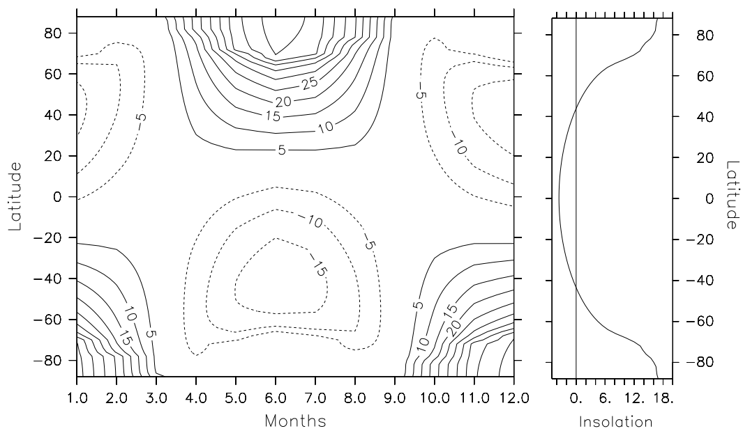
Figure 1: Insolation difference between T_{max} (24.45°) and T_{min} (22.05°). On the left, insolation difference in W/m^2 is given per month on the x-axis and latitude on the y-axis. On the right, annual mean insolation difference is given, in W/m^2 .
