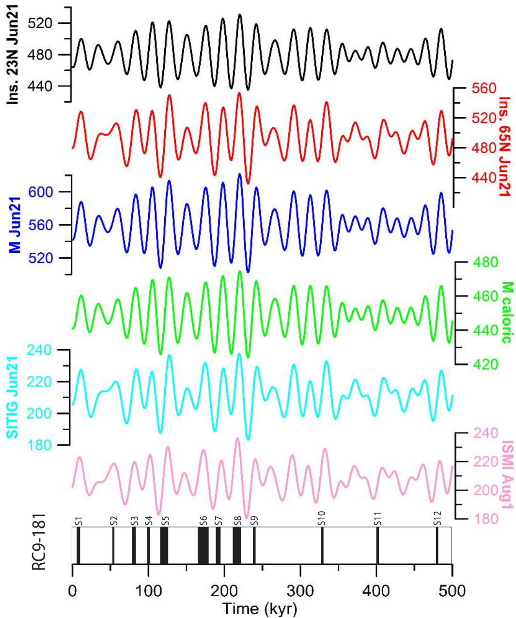
Figure 2: Insolation in W/m^2 over the past 500 kyr at 23^\circ N (black) and 65^\circ N (red) and insolation indices M (blue, green, Rossignol-Strick 1985), SITIG (light blue, Reichart 1996) and ISMI (pink, Leuschner and Sirocko 2003), based on the astronomical solution of Laskar et al. (2004), using Analyseries (Paillard et al., 1996). All are for June 21st, except M caloric (green) which is for the summer half year. The lowest part of the figure shows sapropels in core RC9-181 (Cita et al., 1977; Vergnaud-Grazzini et al., 1977). We note that the obliquity signal also appears in older parts of the insolation and sapropel records (e.g. Lourens et al., 1996; Hilgen et al., 1995, 2003; Zeeden et al., 2014).
