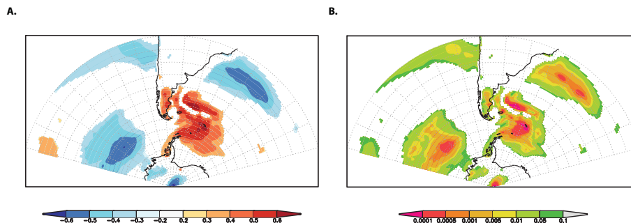
Figure 4. Correlation (a) and significance (b) of relationship between the hemispherically-averaged Southern Annular Mode (SAM) index (Marshall, 2003) with 2 m air temperature in the ERA-79 Interim reanalysis (Dee et al., 2011) (July–June 1979–2013). Analyses were made with KNMI Climate Explorer (van Oldenborgh and Burgers, 2005).
