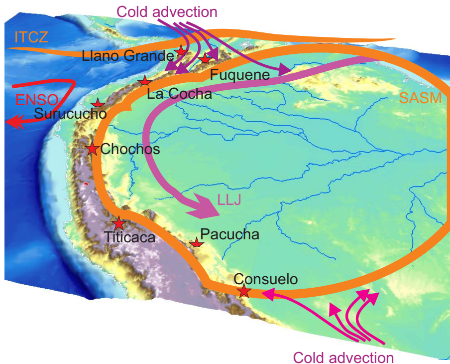
Figure 1. Map showing the Northern and Central Andes and major atmospheric patterns and oceanic systems controlling environmental conditions in the region. ITCZ: intertropical convergence zone, SASM: South American summer monsoon, ENSO: El Niño southern oscillation, LLJ: Low level jet. Red stars show the locations of sites mentioned in the text and described in Table 1.
