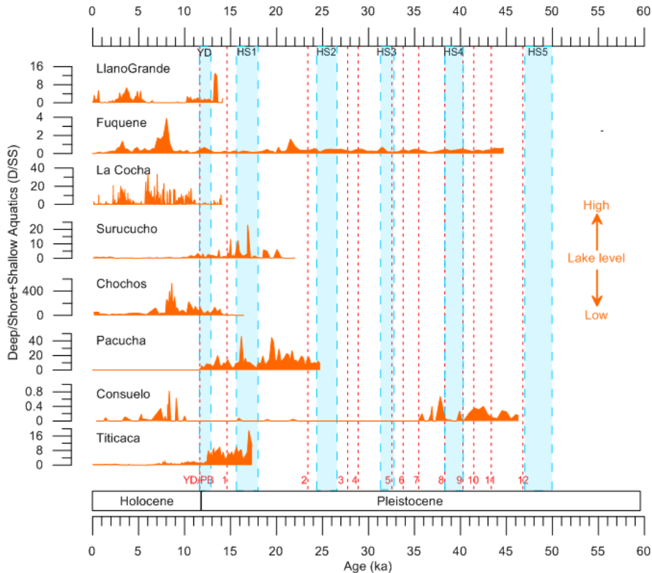
Figure 4. Temporal changes in the ratio of aquatic taxa characteristic of deep water to taxa from shallow water and wet shores (D/SS) for selected sites in the tropical Andes (Fig. 1, Table 1). Heinrich stadials (HS) are drawn for reference as defined by Sánchez-Goñi and Harrison (2010). The Younger Dryas (YD) follows the timing of Greenland stadial 1 (Rasmussen et al., 2006) and the chronozone defined by Mangerud et al. (1974). Red dotted lines and numbers indicate the onset of Greenland interstadials (GI) in Greenland ice cores (Wolff et al., 2010).
