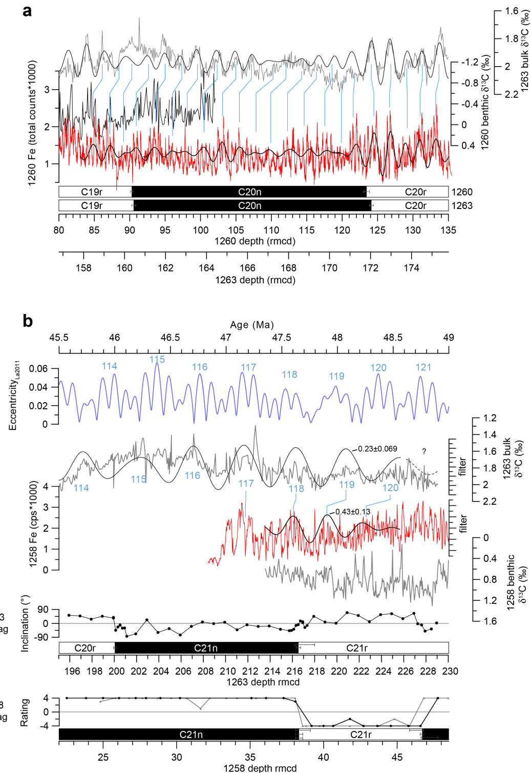
800 Figure 6. Connecting the 405-kyr cyclostratigraphy of ODP Sites 1258 and 1260 with 801 Site 1263. A. Correlation of geochemical and paleomagnetic data from ODP Sites 1263 802 and 1260. Site 1260: benthic \delta^{13}\text{C} in black (25), XRF core scanning Fe intensities in red
