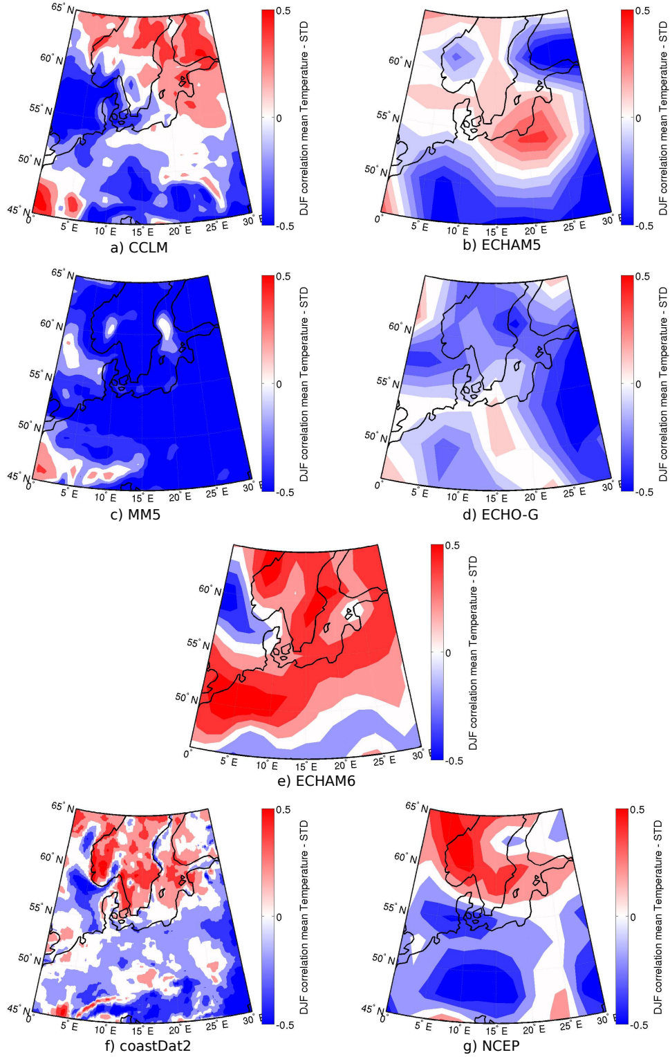
Figure 8: Correlation of between field mean Temperature and STD of wind speed for 7 different data sets in the overlapping time period from 1948 to 1990: a) CCLM, b) ECHAM5, c) MM5, d) ECHO-G, e) ECHAM6, f) coastDat2, g) NCEP
