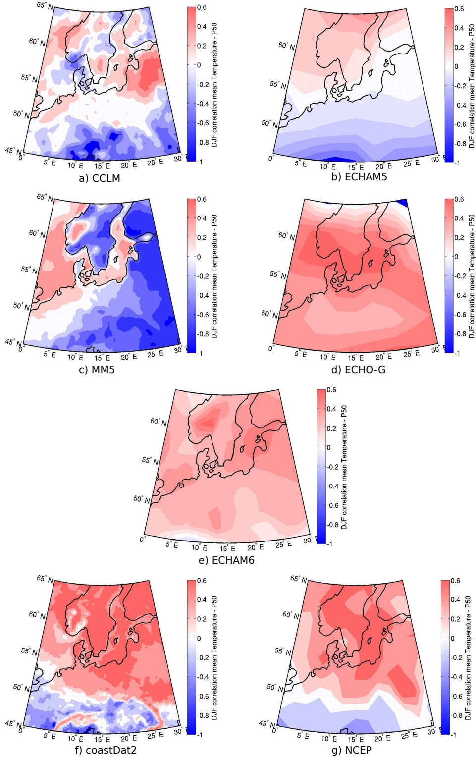
Figure 3: Correlation of between field mean Temperature-temperature and 50th percentile of wind speed for 7 different data sets: a) CCLM (1655-1999 AD), b) ECHAM5 (850-2005 AD), c) MM5 (1001-1990 AD), d) ECHO-G (1001-1990 AD), e) ECHAM6 (850-2005 AD), f) coastDat2 (1948-2012 AD), g) NCEP (1948-2012 AD)
