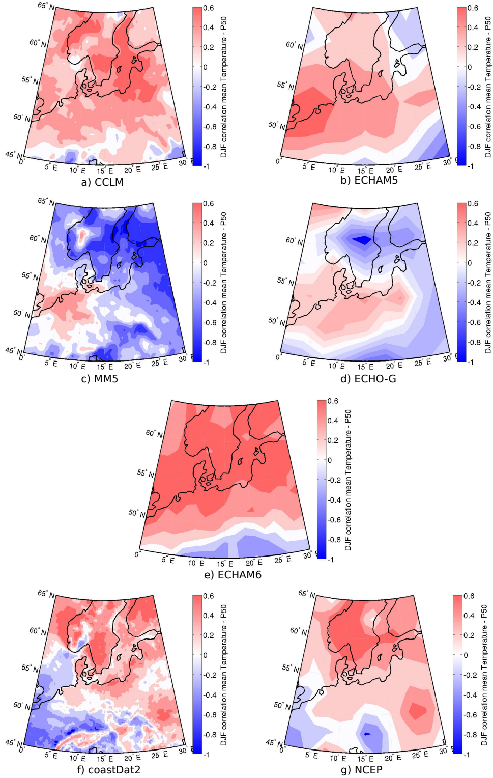
Figure 7: Correlation of between field mean Temperature and 50th percentile of wind speed for 7 different data sets in the overlapping time period from 1948 to 1990: a) CCLM, b) ECHAM5, c) MM5, d) ECHO-G, e) ECHAM6, f) coastDat2, g) NCEP
