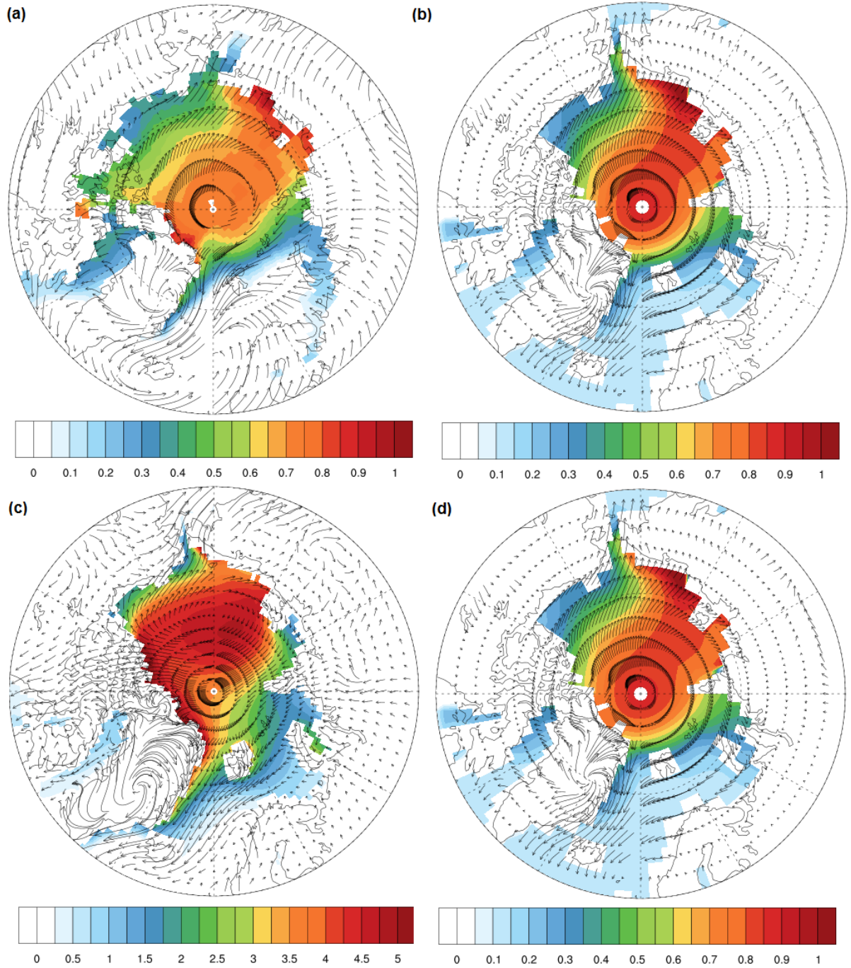
Figure 12. Mean annual 10 m winds and sea ice thicknesses (m) for (a) COSMOS mid-Pliocene, (b) MIROC4m mid-Pliocene, (c) IPSLCM5A pre-industrial and (d) NorESM-L pre-industrial. Vector length is proportional to wind speed.
