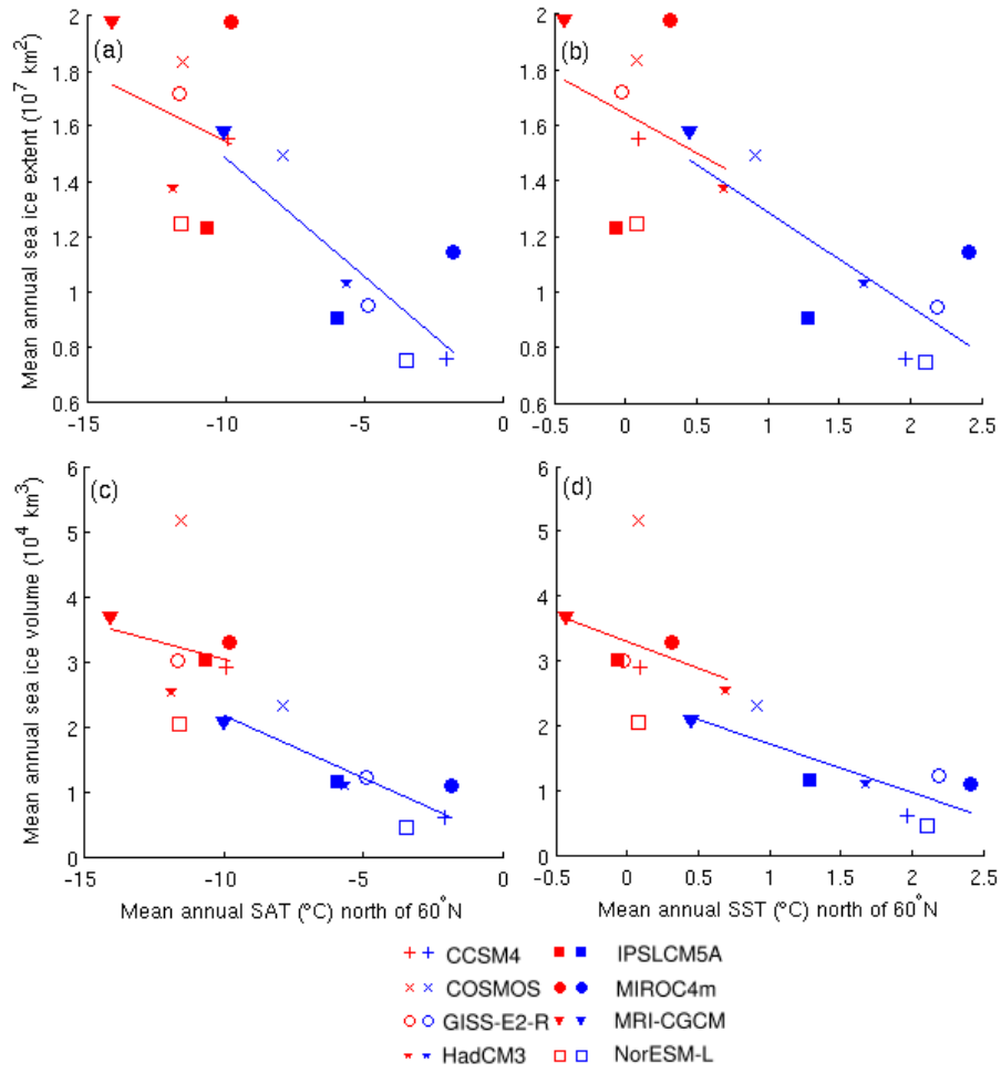
Figure 10. Mean annual surface temperatures north of 60^{\circ}\text{N} vs. mean annual total Arctic sea ice extent(a,b), and mean annual surface temperatures north of 60^{\circ}\text{N} vs. mean annual total Arctic sea ice volume(c,d) in both pre-industrial and mid-Pliocene simulations, for (a,c) SAT and (b,d) SST. Pre-industrial experiments are marked red, mid-Pliocene experiments are marked blue. Correlation coefficients for the pre-industrial simulations in each plot are (a) -0.18, (b) -0.26, (c) -0.12, (d) -0.29. Correlation coefficients for the mid-Pliocene simulations in each plot are (a) -0.76, (b) -0.73, (c) -0.83, (d) -0.82
