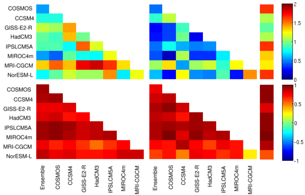
Figure 4. Root-mean-square error (RMSE) (top) and spatial pattern correlations (bottom) of Arctic ice thickness in the pre-industrial (left) and mid-Pliocene (right) simulations by the PlioMIP models and ensemble mean. The single columns to the right show the RMSE and spatial pattern correlations for between each model's pre-industrial and mid-Pliocene mean annual Arctic sea ice thickness.
