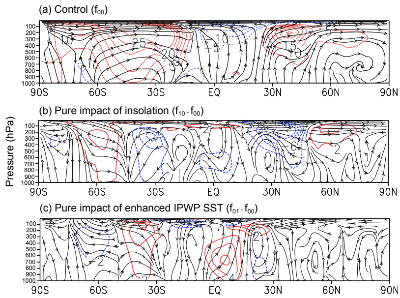
Figure 5. JJA mean meridional wind circulations averaged over 105°E to 120°E. (a) The control experiment ( f_{00} ), (b) the pure impact of insolation ( f_{10}-f_{00} ), and (c) the pure impact of enhanced IPWP SST ( f_{01}-f_{00} ). Stream lines indicate meridional wind circulation for (a) and anomalies for (b) and (c). Contour lines indicate zonal wind circulation or anomalies (with an interval of 5 m/s for (a) and 2 m/s for (b) and (c)).
