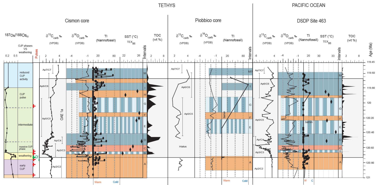
Figure 8. Nannofossil temperature index (TI), TEX 86 , and oxygen-isotope values for the Cismon core, Piobbico core and DSDP Site 463 plotted against chemostratigraphy. The age determination is based on the cyclocronology available for the Cismon core (Malinverno et al., 2010). \delta^{13}\text{C} data after: Erba et al. (1999) and Méhay et al. (2009) for the Cismon core; Erba et al. (under final review by the editor) for the Piobbico core; Price (2003), Ando et al. (2008) and Bottini et al. (2012) for DSDP Site 463. Bulk \delta^{18}\text{O} data after: Erba et al. (2010) for the Cismon core; Price (2003), Ando et al. (2008) and this work for DSDP Site 463. TOC after: Erba et al. (1999) and Bottini et al. (2012) for the Cismon core; Ando et al. (2008) for DSDP Site 463. TEX 86 after: Schouten et al. (2003) for DSDP Site 463; this work for the Cismon core (SST calculated using the equation of Kim et al., 2010). On the left is reported the Os-isotope curve (Bottini et al., 2012) and the volcanogenic CO 2 pulses (red arrows) reconstructed by Erba et al. (2010). The intervals A to M represent the climatic interludes (warming and cooling) reconstructed in this work.
