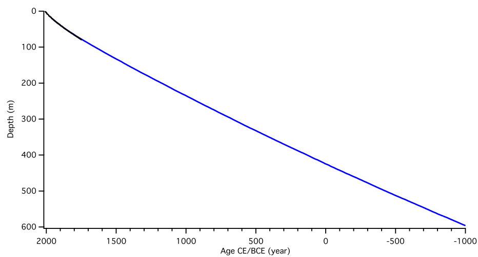
Fig. 1. Figure S7. Age model representation.
