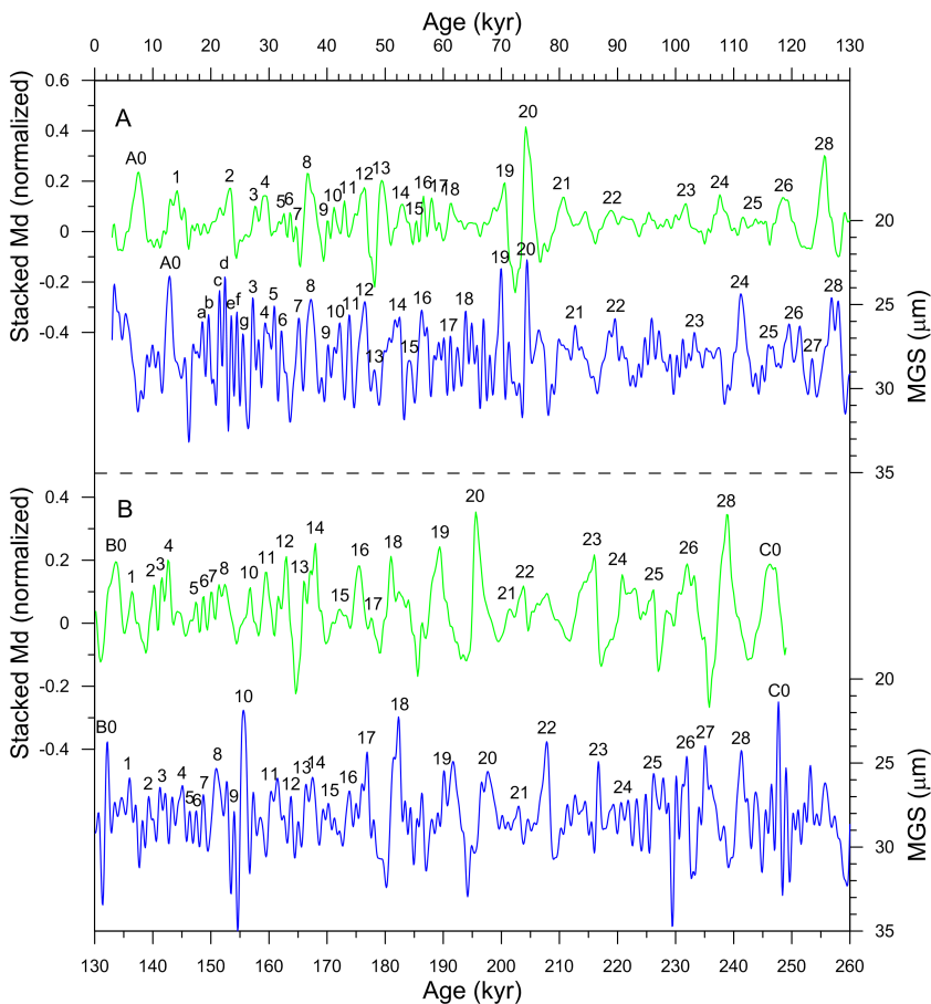
Fig. 2. Fig. 2 Comparison between millennial-scale (filtered 9-1 kyr) variations of Gulang MGS (blue) and the 249kyr grain size stack (green, Yang and Ding, 2014) over the last two glacial-interglacial cycles
