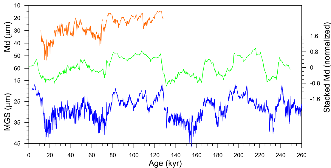
Fig. 1. Fig.1 Comparison of Gulang Mean grain size (MGS, blue) with Shagou median grain size (Md, orange, Wu et al., 2005), and normalized “CHILOMOS” Md (green, Yang and Ding, 2014).
