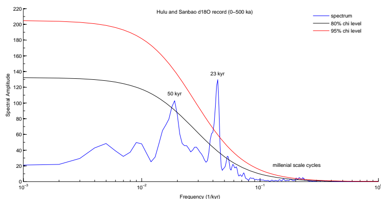
Fig. 1. spectral analyses on the 500 kyr long speleothem d18O record
