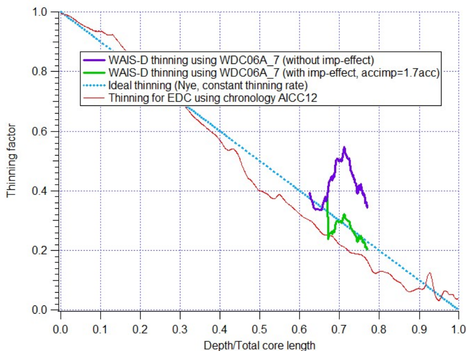
Fig. 1. Thinning function of WAIS-D ice core
