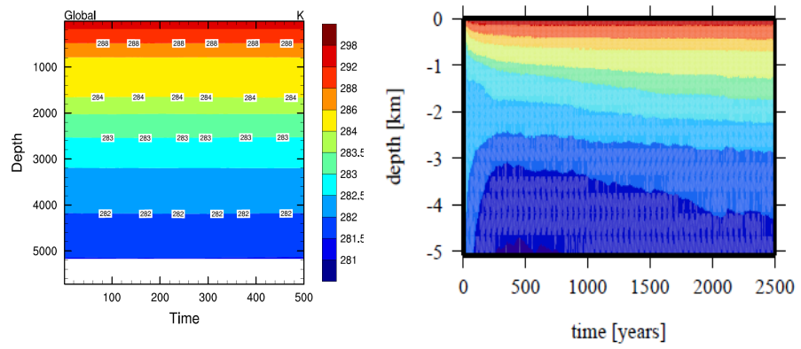
Globally averaged ocean temperature in the stand-alone setup (left, covering 500 years) and for the spin-up of the coupled run (right, covering 2500 years) (Heinemann 2009, dissertation).
