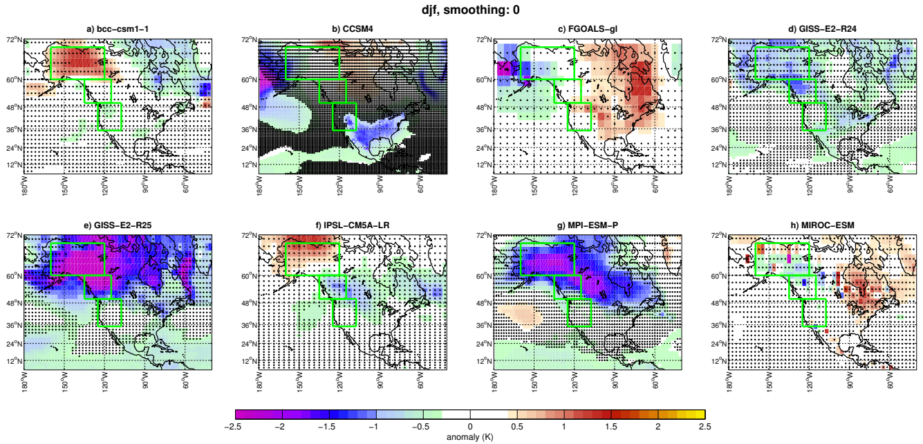
Figure S11 – Winter (djf) surface air temperature anomalies for the period 1800-1820 from the pre-industrial climatology. Dots mark grid points where the anomaly does not exceed the 5 th -95 th percentile range of 21-year running mean anomalies for the pre-industrial period. The select period corresponds to the approximate duration of the early-19 th -century positive PNA phase in the TT2010 reconstruction.
