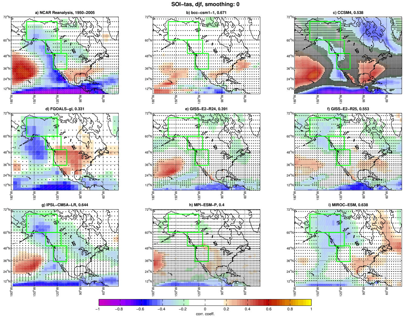
Figure S6 – Observed and simulated correlation maps between the winter SOI index and winter surface-air-temperature time series for the period 1950-2005. Dots mark grid points where the correlation is not significant at 95% confidence accounting for autocorrelation. The green contours mark the boxes used for the TT2010 reconstruction. In panels b-i, the numbers reported in the title are the spatial correlations between observed and simulated patterns calculated for the shown land-only domain north of 12° N (to this purpose NCAR data were regridded to the model grid).
