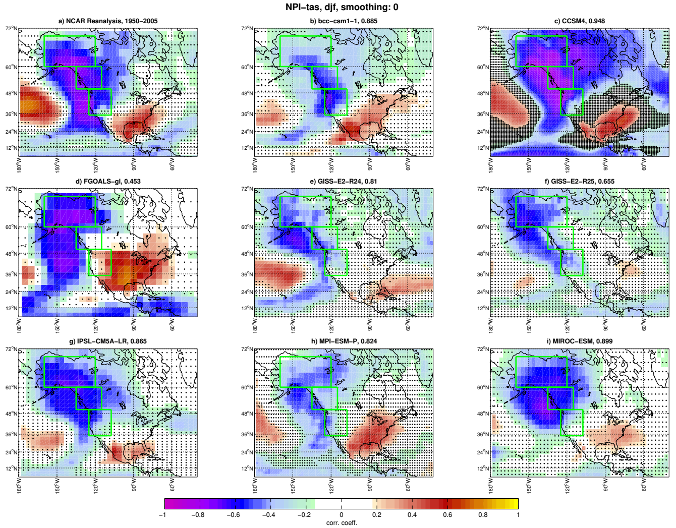
Figure S4 – Observed and simulated correlation maps between the winter NPI index and winter surface-air-temperature time series for the period 1950-2005. Dots mark grid points where the correlation is not significant at 95% confidence accounting for autocorrelation. The green contours mark the boxes used for the TT2010 reconstruction. In panels b-i, the numbers reported in the title are the spatial correlations between observed and simulated patterns calculated for the shown land-only domain north of 12° N (to this purpose NCAR data were regridded to the model grid).
