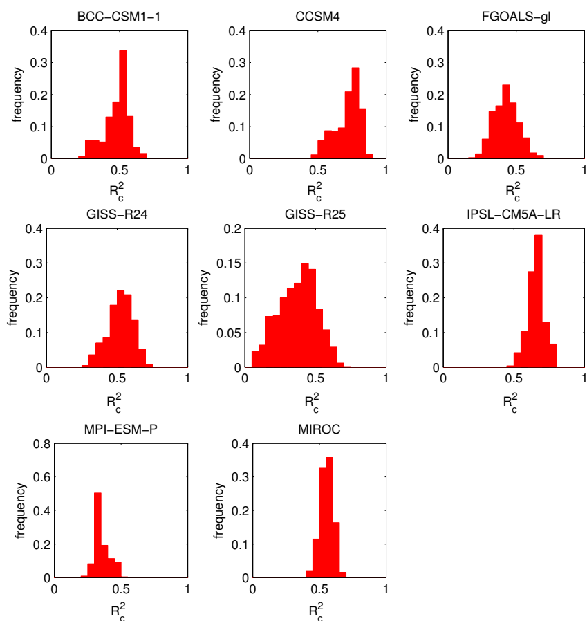
Figure S8 – Empirical probability distributions of calibration R^2 values for the full ensemble of TT2010-like PNA pseudo-reconstructions for individual simulations, from which pseudo-reconstructions illustrated in Figures 7a,b and 8 in the main manuscript are sampled. Note that the y-axis has different scales in the different panels.
