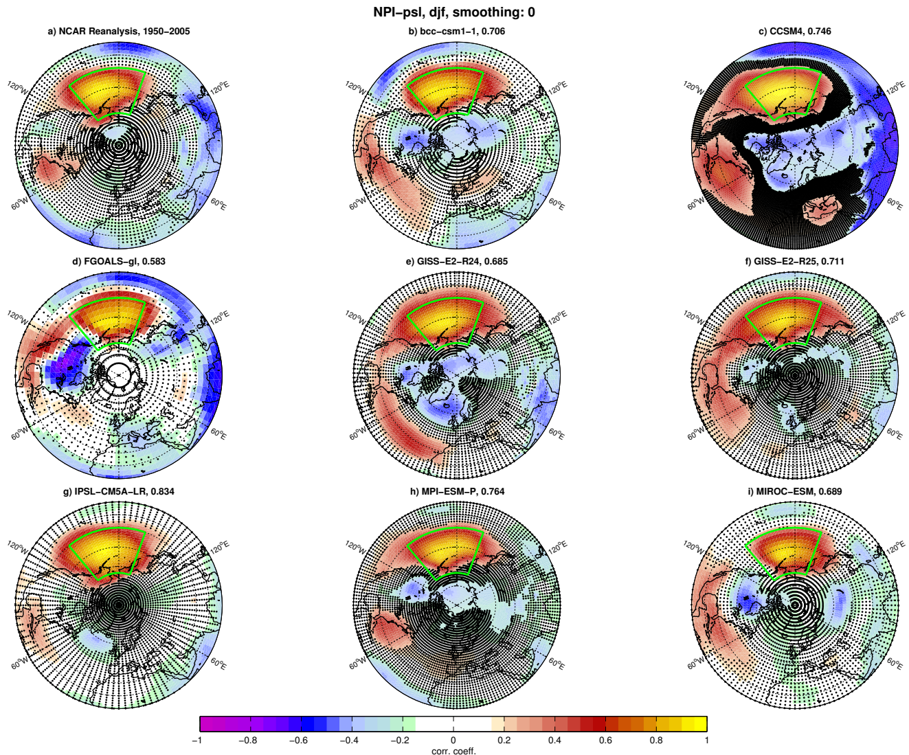
Figure S1 – Observed and simulated correlation maps between the winter NPI index and winter sea-level pressure time series for the period 1950–2005. Dots mark grid points where the correlation is not significant at 95% confidence accounting for autocorrelation. The green contour marks the domain used for the calculation of the NPI index. In panels b–i, the numbers reported in the title are the spatial correlations between observed and simulated patterns calculated for the domain north of 20° N (to this purpose NCAR data were regridded to the model grid).
