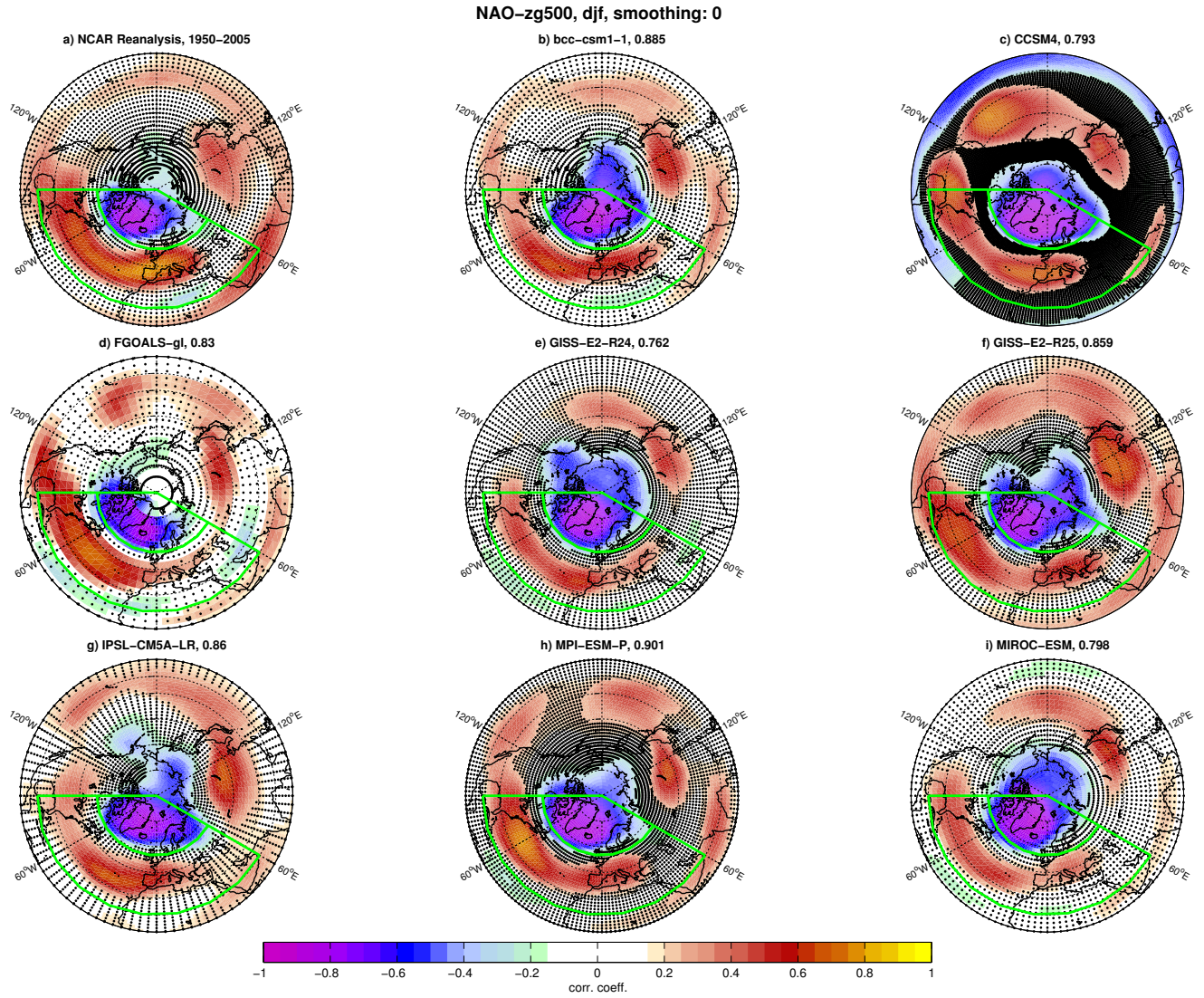
Figure S2 – Observed and simulated correlation maps between the winter NAO index and winter Z500 time series for the period 1950-2005. Dots mark grid points where the correlation is not significant at 95% confidence accounting for autocorrelation. The green contours mark the boxes used for the calculation of the NAO index. In panels b-i, the numbers reported in the title are the spatial correlations between observed and simulated patterns calculated for the domain north of 20° N (to this purpose NCAR data were regridded to the model grid).
