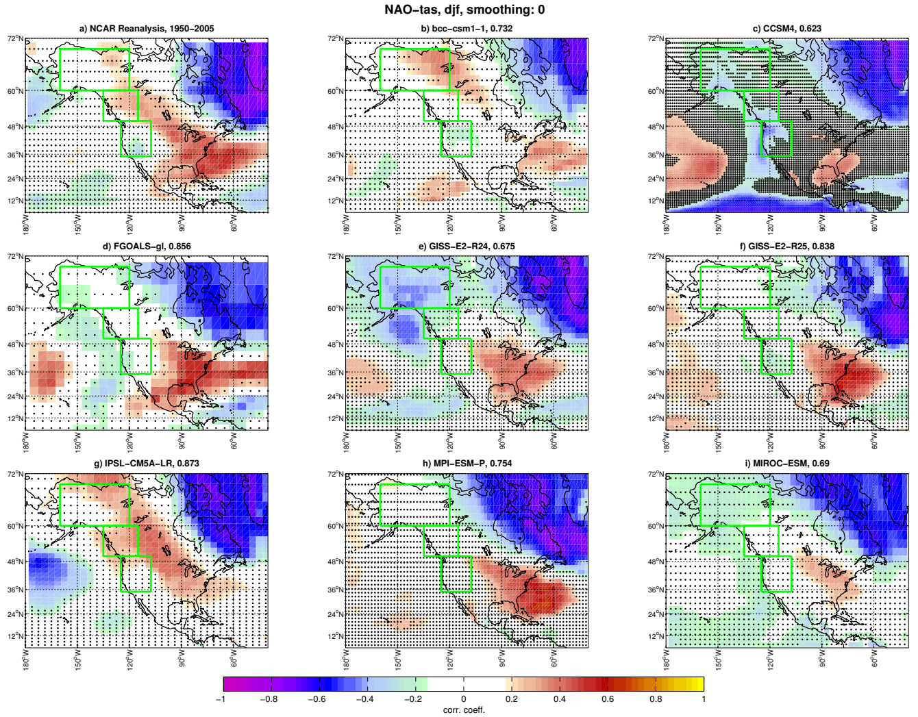
Figure S5 – Observed and simulated correlation maps between the winter NAO index and winter surface-air-temperature time series for the period 1950-2005. Dots mark grid points where the correlation is not significant at 95% confidence accounting for autocorrelation. The green contours mark the boxes used for the TT2010 reconstruction. In panels b-i, the numbers reported in the title are the spatial correlations between observed and simulated patterns calculated for the shown land-only domain north of 12° N (to this purpose NCAR data were regridded to the model grid).
