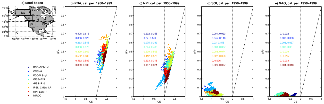
Figure S10 - Skill metrics for an ensemble of TT2010-like reconstructions following Figure 7a: a) map of the three boxes from where gridded data are sampled to be included as predictors, with the name reported in each box (tas: surface air temperature, pr: precipitation); b-e) full-validation period coefficient of determination ( R^2v ) and coefficient of error (CE) for the reconstructions using respectively the winter PNA (b), NPI (c), SOI (d) and NAO (e) as predicted variable. For each reconstruction, the regression model is always calibrated on PNA, see methods. To be comparable with TT2010, only the subset of reconstructions with R^2 for the PNA for the 1950-1999 calibration period in the range [0.45-0.55] are considered ( R^2c=0.49 in TT2010). The numbers inside each panel indicate the minimum and maximum R^2v values obtained for each model.
