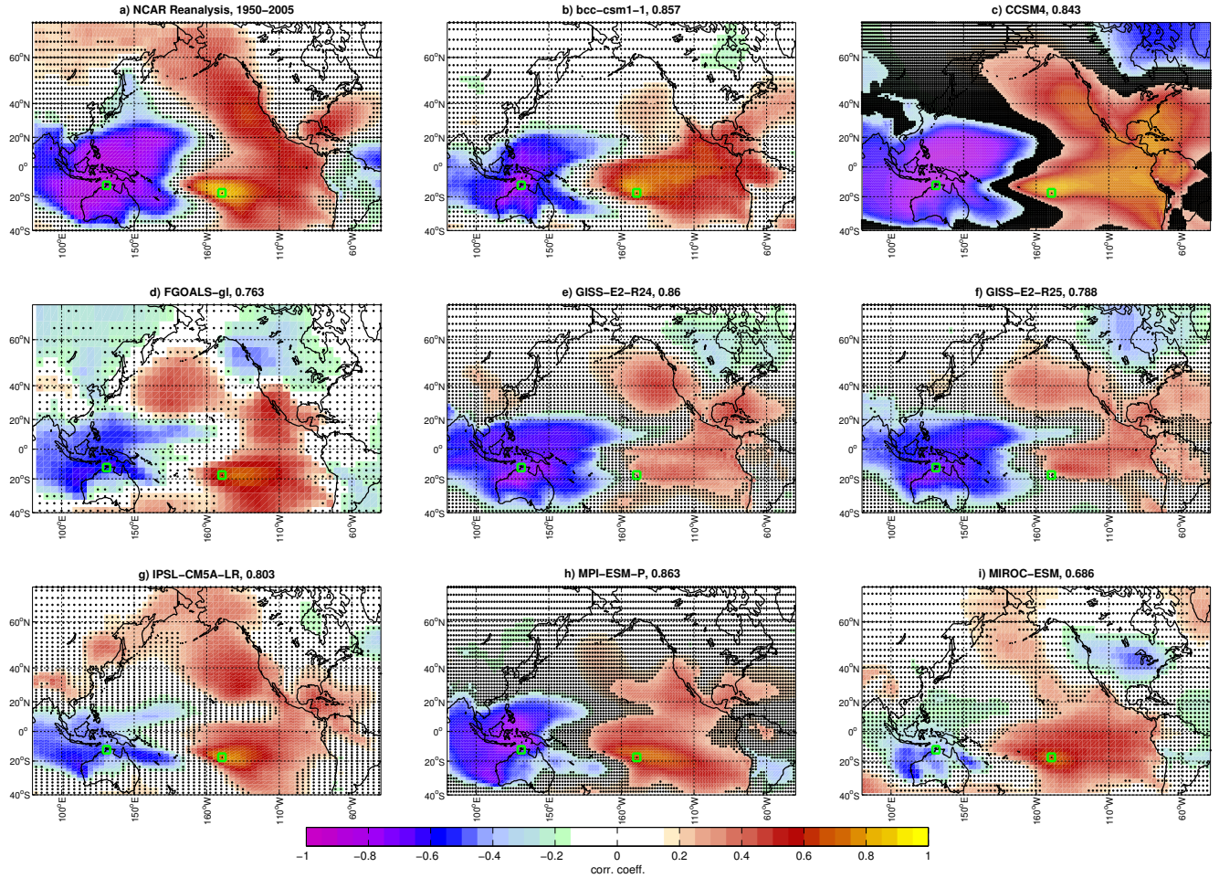
Figure S3 – Observed and simulated correlation maps between the winter SOI index and winter sea-level pressure time series for the period 1950-2005. Dots mark grid points where the correlation is not significant at 95% confidence accounting for autocorrelation. The green contours mark the boxes used for the calculation of the SOI index. In panels b-i, the numbers reported in the title are the spatial correlations between observed and simulated patterns calculated for the shown domain north of 30° S (to this purpose NCAR data were regridded to the model grid).
