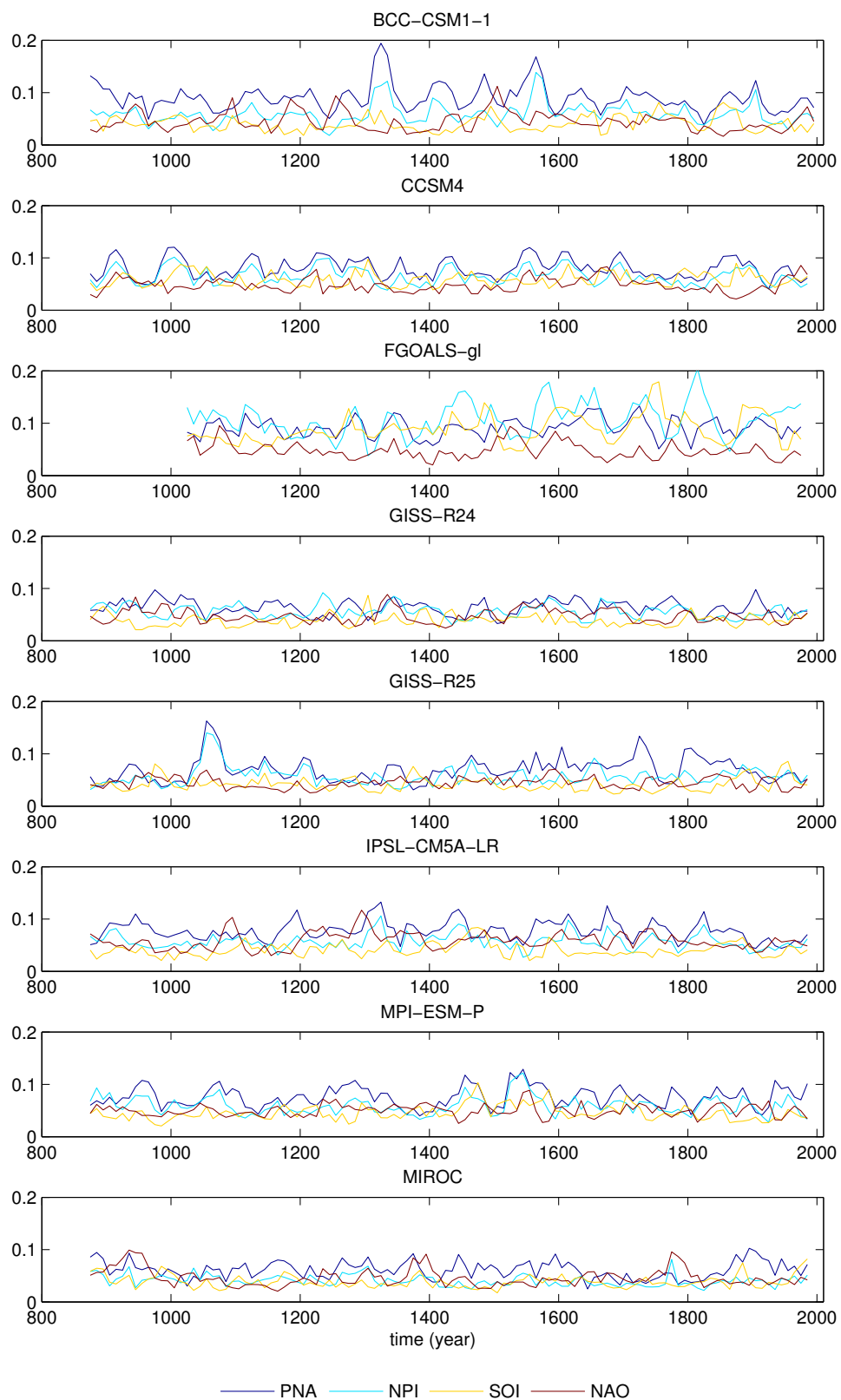
Figure S7 – Fractions of total variance of winter North American precipitation (land only grid points within the domain 20-70°N, 190-300°E) explained by winter PNA, NPI, NAO and SOI indices for individual simulations. Values are calculated over decadal-paced 30-year periods.
