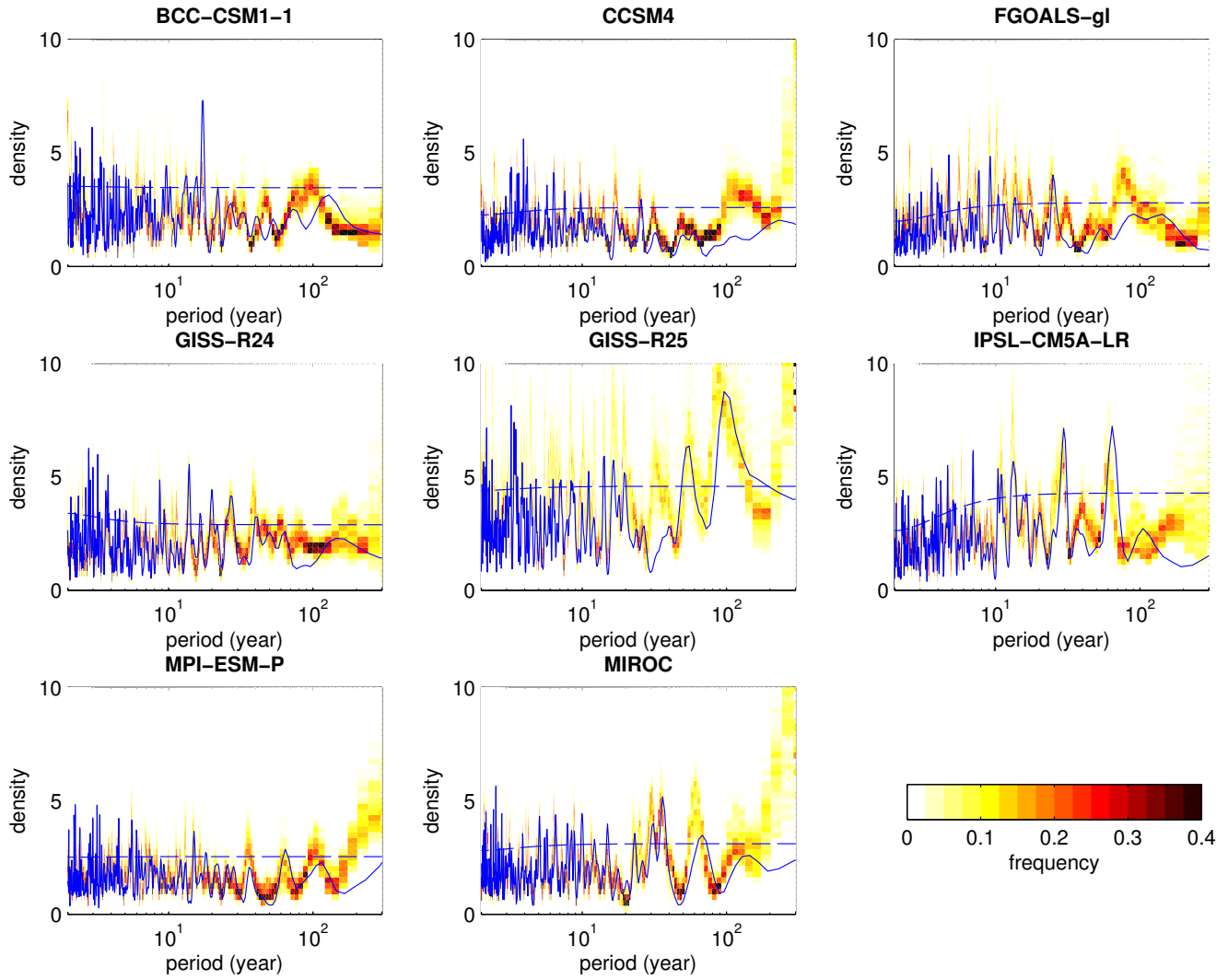
Figure S12 - Power spectral density of the winter PNA index (blue line) for individual simulations with associated 95% confidence level (blue dashed line) and agreement between the spectra of the pseudo-reconstructions obtained following the modified TT2010 approach (including a box over Florida and extended calibration period) and illustrated in Figure 7c of the main paper. All indices are standardized according to the 1950-1999 climatology.
