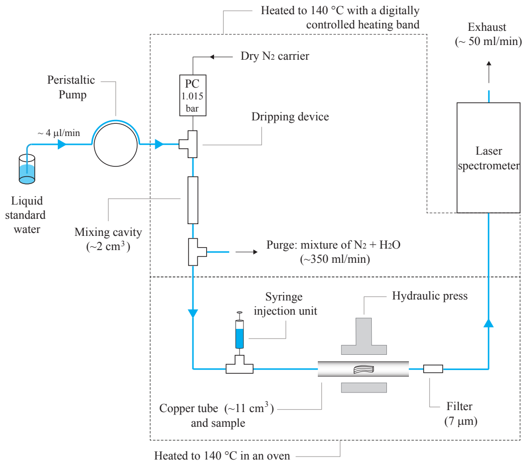
Fig. 1. Diagram of the speleothem fluid inclusions water extraction line.
