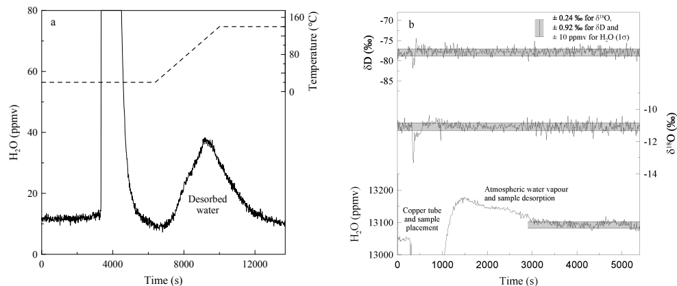
Fig. 3. (a) Desorption test: the large peak corresponds to ambient water vapour migration during the opening of the line when loading the sample. After closing, the sample is flushed with a dry nitrogen stream without heating. After reaching the dry background level the system is heated to 140 °C to desorb the water from the calcite. (b) Example of desorption and stabilisation of water vapour amount and its isotopic composition after loading the sample. Desorption from the sample surface or from fluid inclusion cracks is hardly visible at this resolution.
