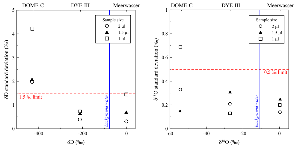
Fig. 11. Summary of the reproducibility tests made for different standard waters ranging from 0 to -450\text{‰} for \delta D (left panel) and from 0 to -55\text{‰} for \delta^{18}O (right panel).
