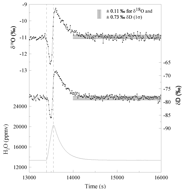
Fig. 8. These spectrograms show the \delta^{18}\text{O} , \delta\text{D} and \text{H}_2\text{O} responses of the Picarro for a speleothem sample measurement (Fig. 7, peak 4). Both isotope ratios behave similarly. Due to diffusional fractionation of the light and heavy water isotopologues during the sample transfer by nitrogen, depleted values are observed for the very first part of the sample. Maximal isotope values are reached after the maximum of the water amount. The signals reach background stability again after about 20 min.
