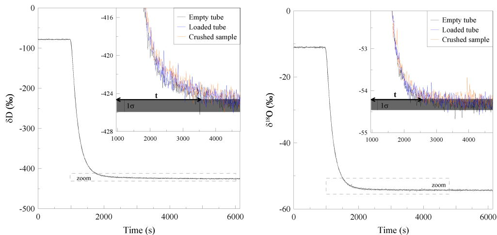
Fig. 6. System response for switching from ST-08 to DOME-C standard water. No difference is noticeable for empty, loaded or crushed tube conditions.
