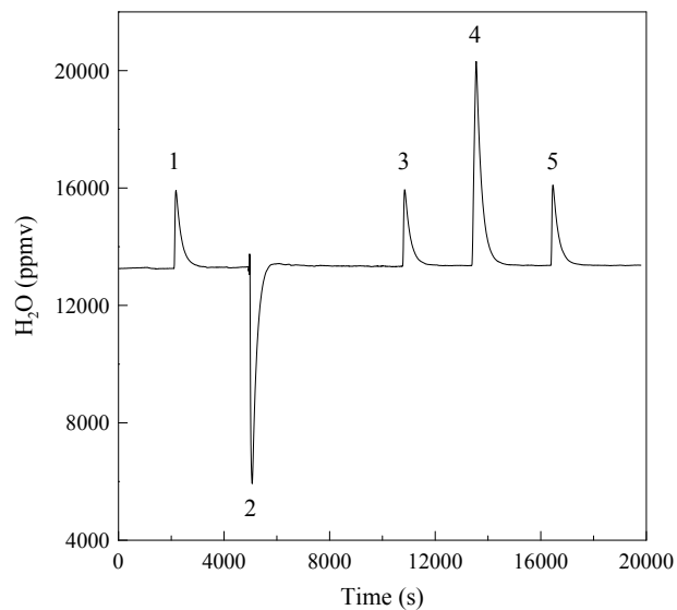
Fig. 7. Water vapour evolution during a measurement sequence. Peaks 1, 3 and 5 are 0.5 \mu\text{L} injections of ST-08 standard water. Peak 4 corresponds to the released fluid inclusion water. The depression 2 corresponds to the exchange between the empty and the loaded copper tube.
