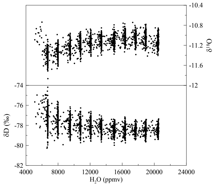
Fig. 5. \delta^{18}\text{O} and \delta\text{D} dependence on injected water vapour amounts presented in Fig.4.
