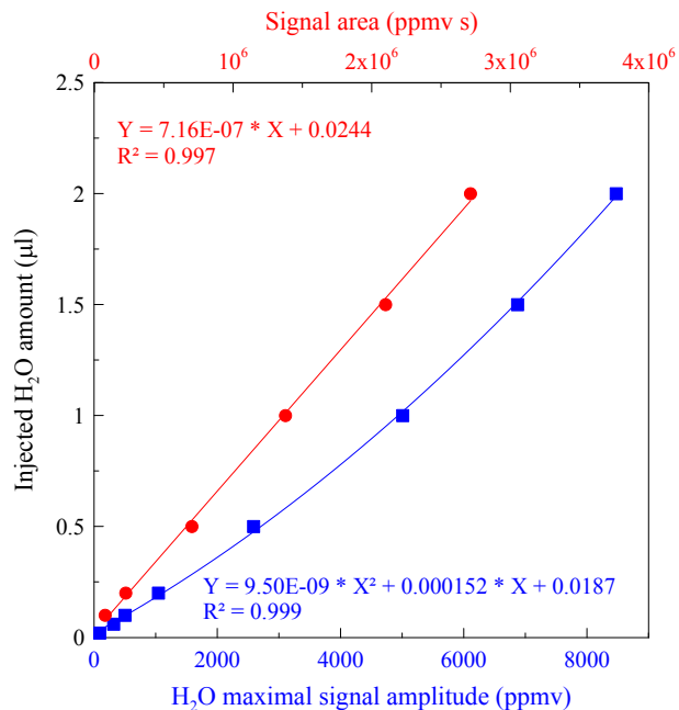
Fig. 9. The relationship between the sample signal and the injected water amount is used to calibrate the released water amount from fluid inclusions. Calibration was determined for amounts up to 2 µL using wet background and based on two schemes: (i) with the signal area converted into water amounts (linear regression in red) and (ii) relative to the maximal signal intensity (polynomial regression in blue).
