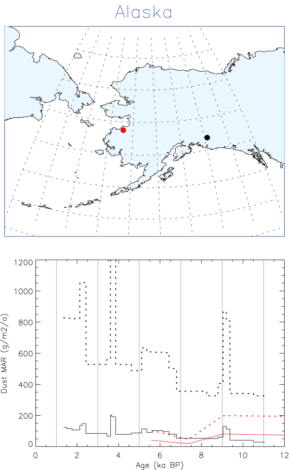
Figure 9. Same as Fig. 6, for Alaska.
