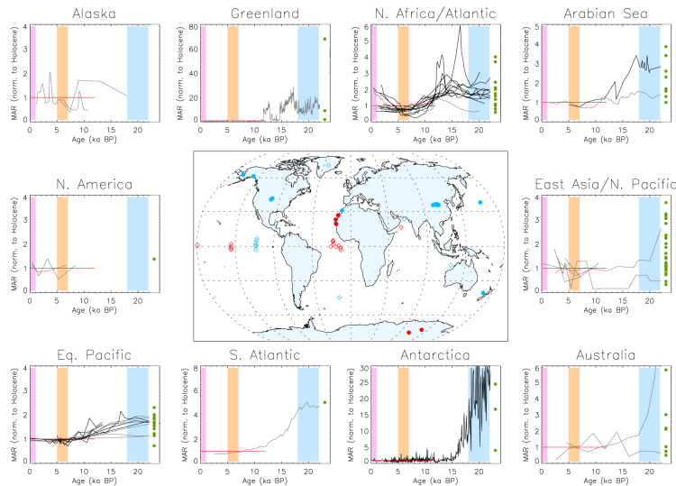
Figure 5. Overview of the data compilation. Central plot: global overview of the location of the paludust records. Color indicates the confidence level (red = high confidence, orange = medium confidence). Marker's shape indicates if size distributions/classes are available (filled circles = yes, empty diamonds = no). Framing plots: time series of bulk dust MAR in the different areas, normalized to their Holocene (0–12 ka BP) average (red solid line for reference, which represents the time span over which DMARs were averaged in the original DIRTMAP: Kohfeld and Harrison, 2001). Black solid lines represent high confidence records; gray lines identify medium confidence records. Records are plotted in the 0–22 ka BP interval, to allow a comparison with DIRTMAP3 (Maher et al., 2010) data (as reported in Albani et al., 2014), represented by their glacial/interglacial ratio (green solid circles). Vertical color shading bands highlight the last millennium (pink), the MH (5–7 ka BP, salmon), and Last Glacial Maximum (18–22 ka BP, light blue).
