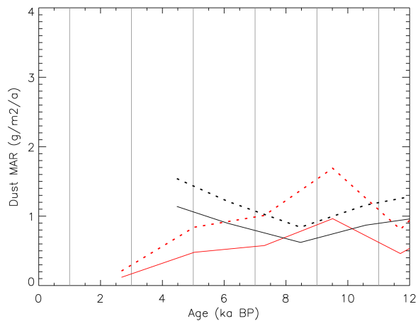
Figure 13. Same as Fig. 6, the Australian region.
