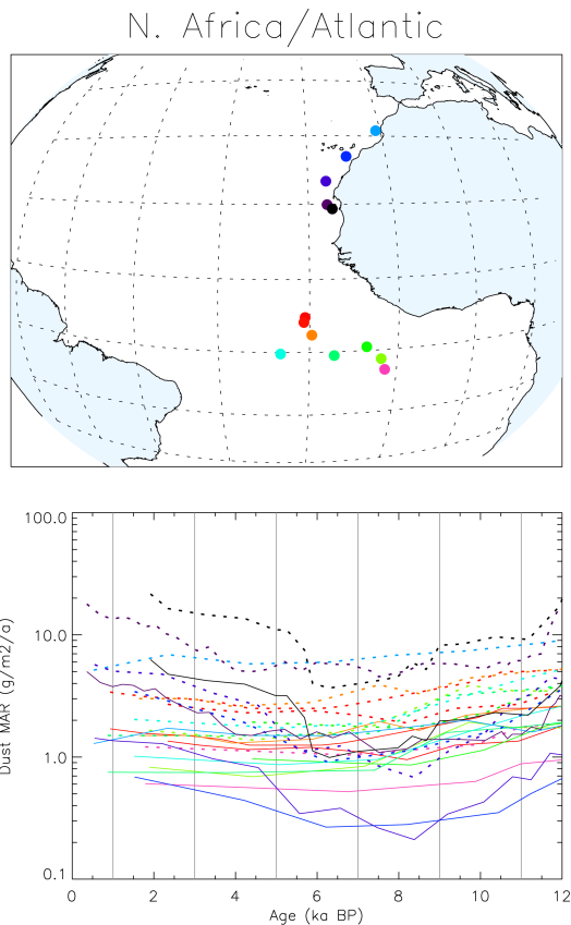
Figure 6. Detailed view of the dust records in the North Africa/North Atlantic region. Upper panel: geographical location of the paleodust records. Bottom panel: time series of the bulk (dotted lines) and “fine” i.e. < 10 μm (solid lines) dust MARs. Color-coding is consistent between upper and lower panel. Vertical grey solid lined mark the sub-periods within the Holocene as described in Sect. 3.4 with a pace of 2 ka.
