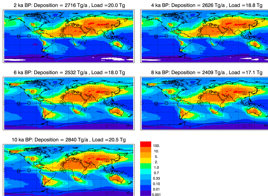
Figure 17. Dust deposition flux ( \text{gm}^{-2} \text{a}^{-1} ) from the CESM during the Holocene snapshots at 2, 4, 6, 8, and 10 ka BP, based on spatially variable emissions constrained by the observational Mass Accumulation Rates. Black circles mark the locations of the observational records in this compilation.
