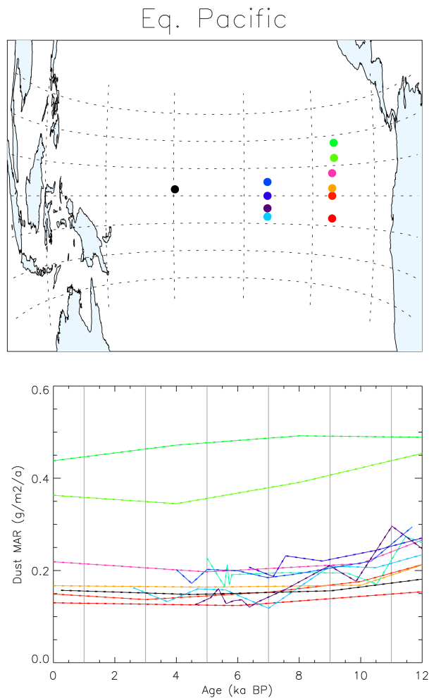
Figure 12. Same as Fig. 6, for the Equatorial Pacific.
