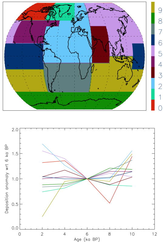
Figure 4. Upper panel: subdivision of the globe in different areas, based on the spatial distribution of data in this compilation (0 = Alaska, 1 = Greenland, 2 = North Africa and North Atlantic, 3 = Arabian Sea, 4 = North America, 5 = East Asia and North Pacific, 6 = Equatorial Pacific, 7 = South Atlantic, 8 = Antarctica, 9 = Australia). Bottom panel: time series (at a 2 ka pace) of the dust deposition anomaly with respect to 6 ka BP for the different areas, as estimated from the observations. Color-coding of the different areas is coherent between upper and lower panel.
