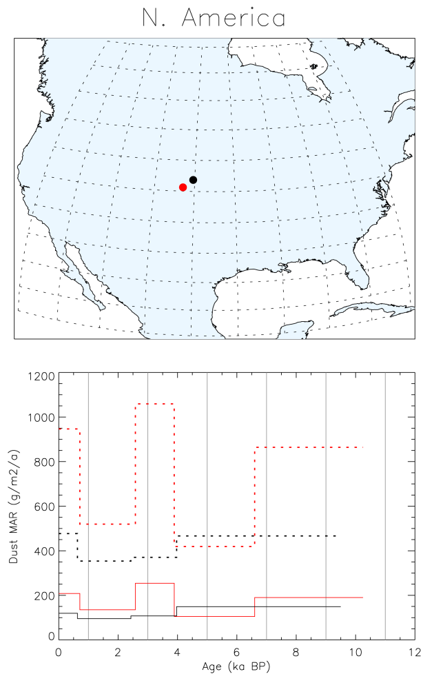
Figure 8. Same as Fig. 6, for the North American region.
