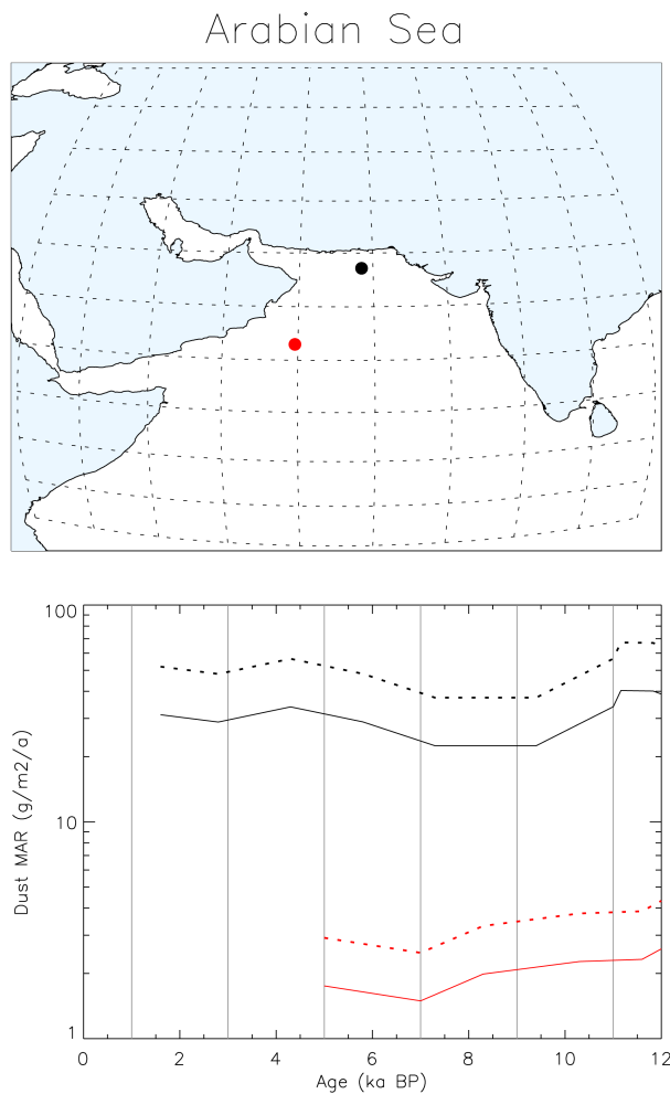
Figure 7. Same as Fig. 6, for the Arabian Sea region.
