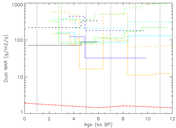
Figure 10. Same as Fig. 6, for East Asia and the North Pacific Ocean.
