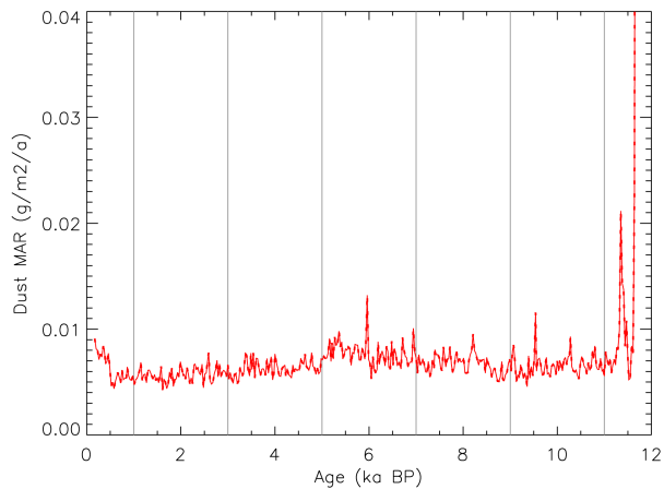
Figure 11. Same as Fig. 6, for Greenland.
