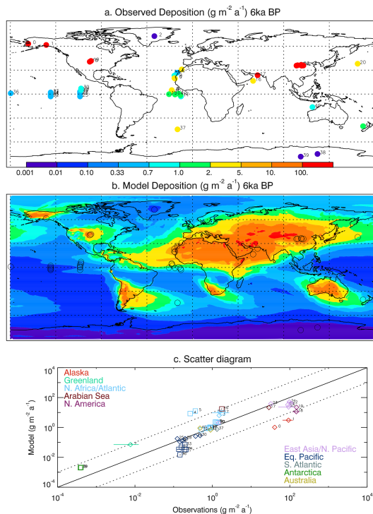
Figure 16. Comparison of simulated dust deposition ( \text{g m}^{-2} \text{a}^{-1} ) for the 6 ka BP case, compared to observational estimates of the fine ( < 10 \mu\text{m} ) eolian Mass Accumulation Rate for the period 5–7 ka BP. (top) Observations; (middle) model; (bottom) model vs. observations scatterplot. Horizontal bars represent the variability of observational data averaged within the 5–7 ka BP time lapse (1 sigma). Locations of observational sites are clustered in the scatterplots based on their geographical location, as indicated by the color-coding. In the bottom scatterplot, squares indicate high confidence level, diamonds represent medium confidence level.
