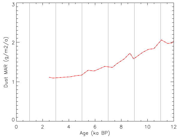
Figure 14. Same as Fig. 6, for the South Atlantic Ocean.
