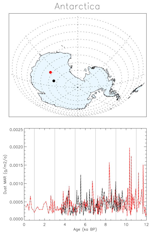
Figure 15. Same as Fig. 6, for Antarctica.
