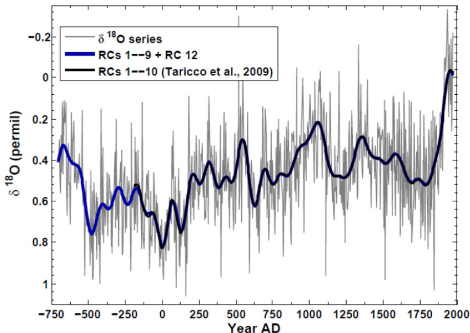
Figure 1. \delta^{18}\text{O} profile (707 BC–1979 AD) measured in the Ionian GT90/3 core (gray line). In order to agree in tendency with temperatures, the isotopic ratio is plotted “upside-down”. The sampling interval is \Delta t = 3.87\text{y} , the raw data mean is x_m = 0.47\text{‰} and their standard deviation is \sigma = 0.23\text{‰} . \delta^{18}\text{O} signal reconstruction obtained by summing up its first 12 significant components extracted by SSA (blue line). The signal reconstruction obtained from the SSA analysis of the shorter, previously published, \delta^{18}\text{O} time series (Taricco et al., 2009) is shown as a black line. Except for a negligible border effect, the agreement between the two smooth curves is excellent over their common section ( r = 0.99 ).
