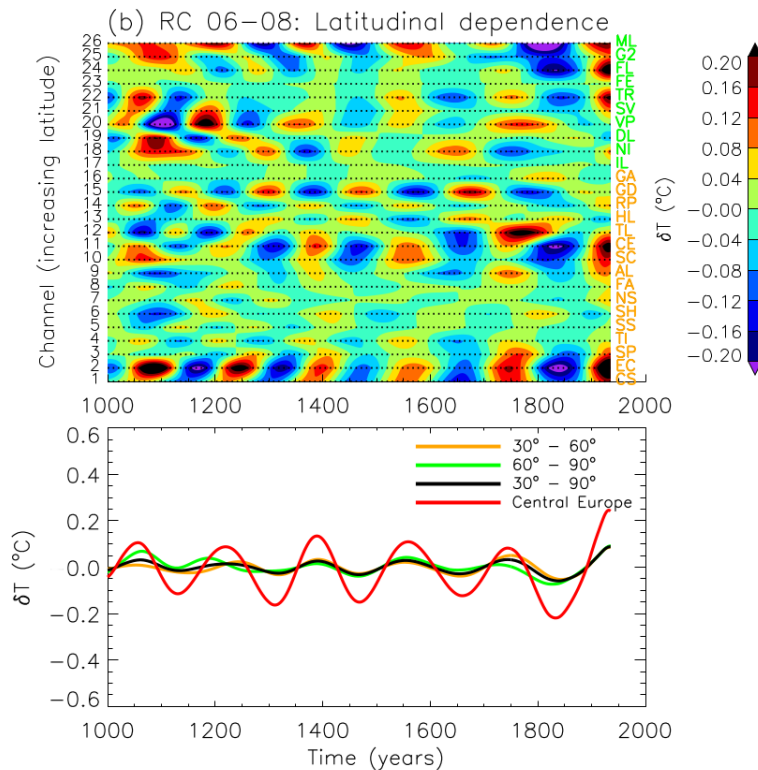
Figure 6. Reconstructed components RCs 6–8 of the NH temperature data set, representing a bicentennial oscillation; color bar for amplitude from -0.20 to 0.20 ^{\circ}\text{C} . Upper-half panel: RC pair of temperature anomalies from MSSA analysis as a function of increasing latitude; lower-half panel: the same RC pair averaged over two latitude bands, namely, 30 – 60^{\circ} N (orange) and 60 – 90^{\circ} N (green), as well as over the entire NH (black). The red curve represents the bicentennial oscillation of the Central Europe series.
