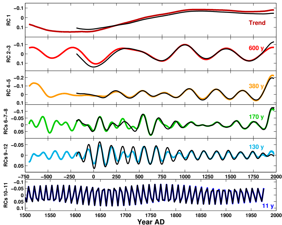
Figure 3. Significant components extracted by SSA from the \delta^{18}\text{O} record: RC1 (trend), RC 2–3 (600 yr), RC 4–5 (380 yr), RCs 6–8 (170 yr), RCs 9–12 (130 yr), and RCs 10–11 (11 yr). The black curves represent the reconstructions of the same oscillations provided by the analysis of the shorter, previously published, \delta^{18}\text{O} time series (Taricco et al., 2009).
