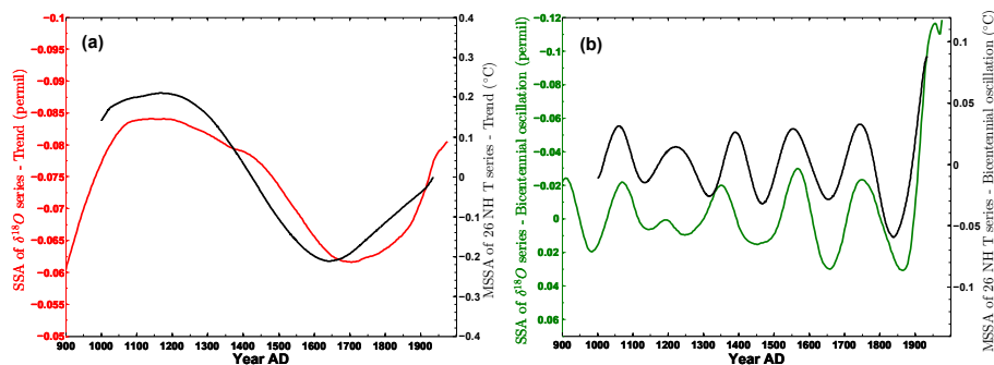
Figure 7. Comparison between the reconstructed components extracted by SSA from the \delta^{18}\text{O} profile and the corresponding oscillations extracted by MSSA from the NH temperature data set. (a) Long-term trend: \delta^{18}\text{O} RC 1 (dark-red line) and NH temperature RCs 1–2 (black line); (b) 170 yr oscillation: \delta^{18}\text{O} RCs 6–8 (green line) and NH temperature RCs 6–8 (black line).
