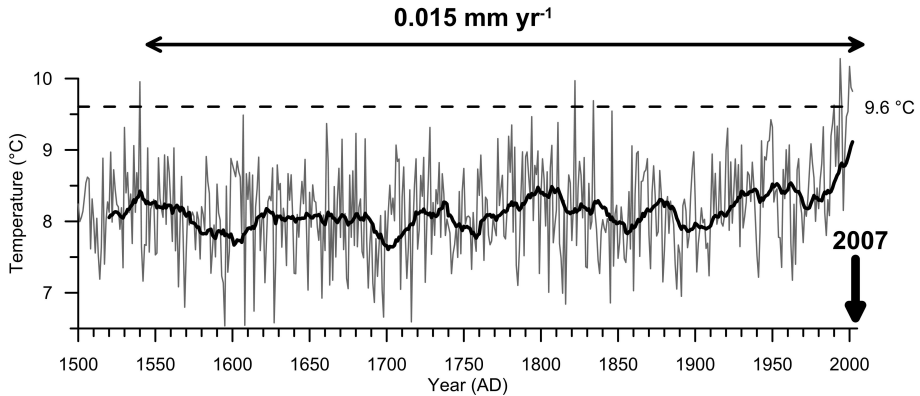
Figure 6. Surface temperature reconstruction (47-48° N; 6.5-7.5° E; Luterbacher et al. (2004)). The grey graph shows the annual temperatures, a 20 yr running average is plotted in black. The current cave temperature is shown as a dashed line. The black horizontal arrow denotes the estimated temporal coverage of the studied 6 mm long section of stalagmite M2 assuming an average growth rate of 0.015 mm per year. The vertical black arrow denotes the age of the top (date of sampling) of stalagmite M2.
