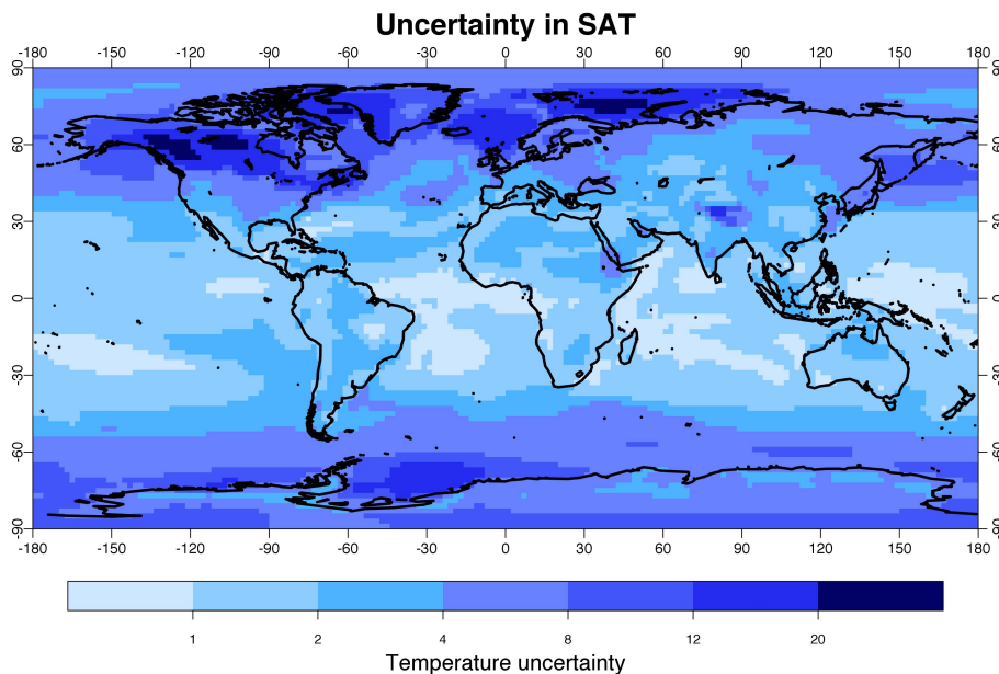
Fig. 3. Uncertainty in Last Glacial Maximum surface air temperature ( ^{\circ}\text{C} ) from bootstrap resampling. Results presented as half-width of 95% confidence interval.
