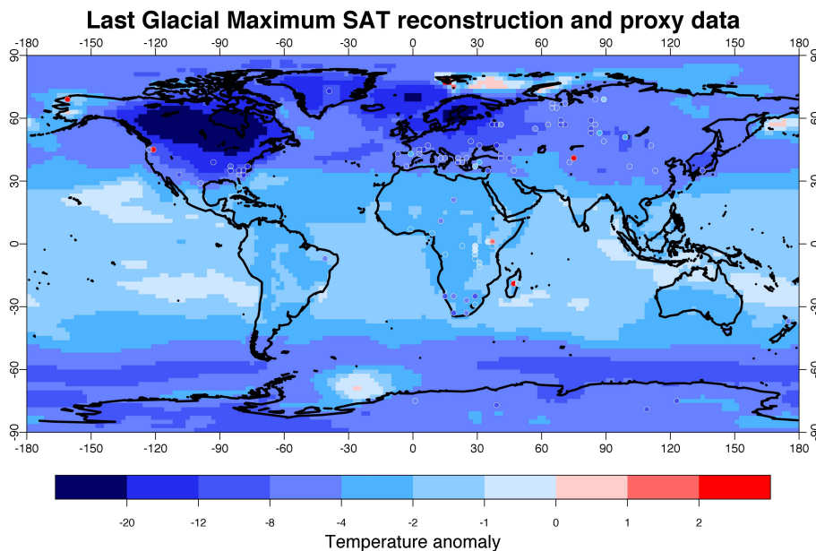
Fig. 1. Reconstruction of Last Glacial Maximum surface air temperature ( ^{\circ}\text{C} ) based on multi model regression. Proxy data are represented as coloured dots.
