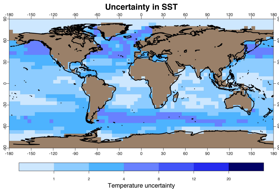
Fig. 4. Uncertainty in Last Glacial Maximum sea surface temperature ( ^{\circ}\text{C} ) from bootstrap re-sampling. Results presented as half-width of 95 % confidence interval. Land areas are masked as brown.
