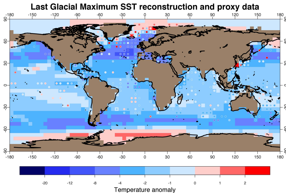
Fig. 2. Reconstruction of Last Glacial Maximum sea surface temperature ( ^{\circ}\text{C} ) based on multi model regression. Proxy data are represented as coloured dots. Land areas are masked as brown.
