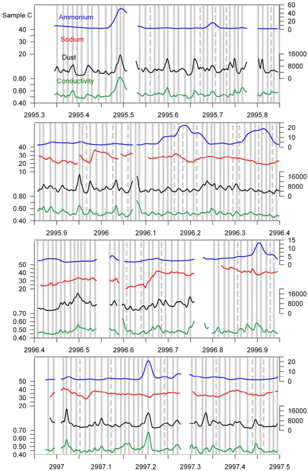
FIGURE S3. Measured profiles for sample 'C'. Units and annual layer counting as in Fig. 5.
