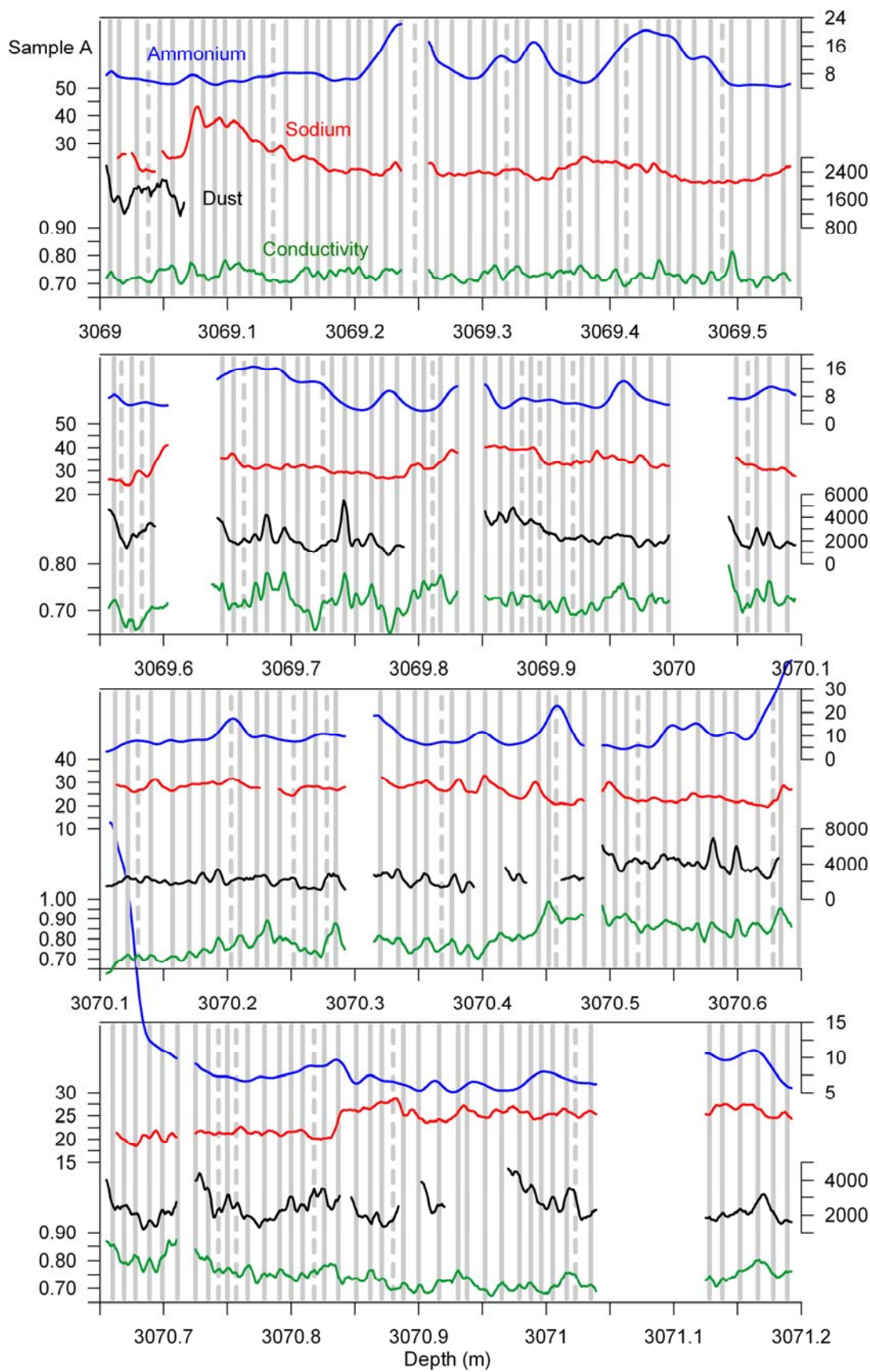
FIGURE S1. Measured profiles for sample 'A'. Units and annual layer counting as in Fig. 5.
