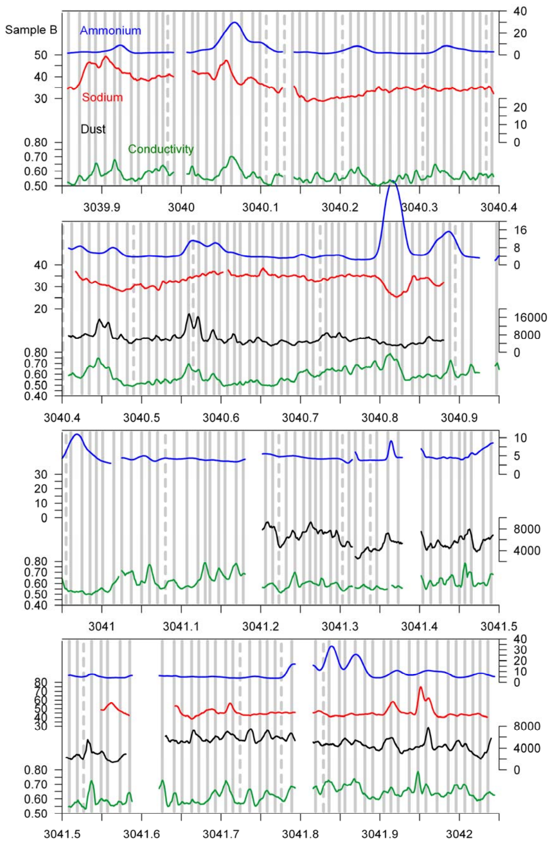
FIGURE S2. Measured profiles for sample 'B'. Units and annual layer counting as in Fig. 5.
