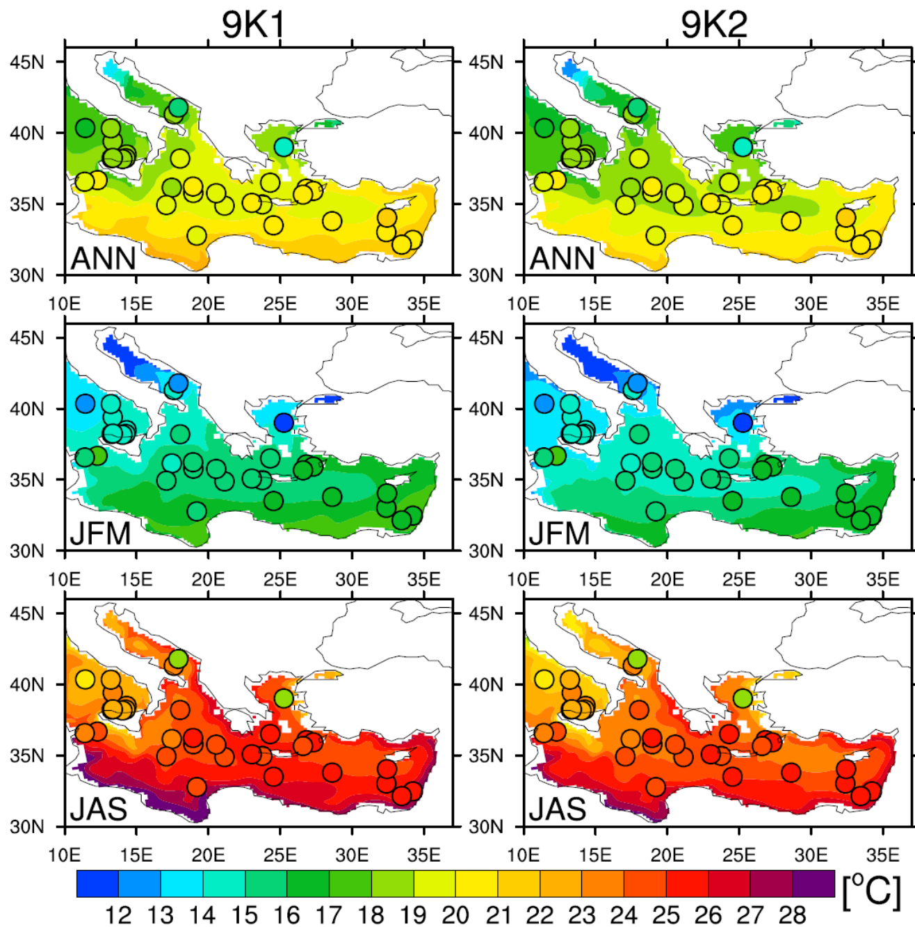
Fig. S2: Annual, winter (JFM) and summer (JAS) SSTs, reconstructed from proxy data (dots, Kucera et al., 2011) vs. modelled one (background color) for 9K1 (left) and 9K2 (right). 1st row displays annual SST, 2nd row displays winter SST, 3rd row displays summer SST.
