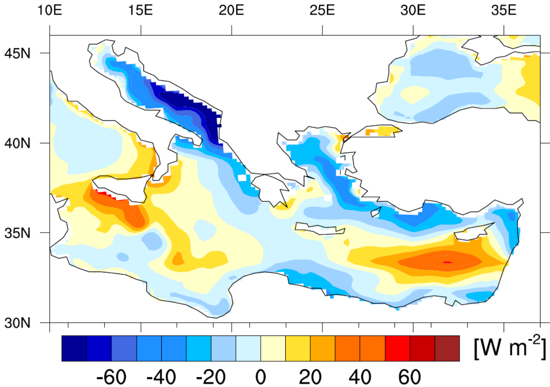
Fig. S1: Annual mean net heat flux at the surface for CTRL.
