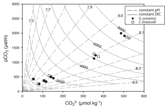
Fig. 1. The carbonate chemistry conditions ( \text{CO}_3^{2-} in \mu\text{mol/kg} and p\text{CO}_2 in \mu\text{atm} ) as measured at the beginning of each of our incubations for G. oceanica (black dots) and C. braarudii (open squares). Contours of constant pH with increasing DIC are indicated by the dashed grey lines whereby saturation state (proportional to \text{CO}_3^{2-} since all experiments were run at constant Ca concentration of 10 mmol/kg) and p\text{CO}_2 are positively correlated in our experiments. By contrast, the majority of previous experiments follow the solid grey curves at constant DIC but with varying pH which results in an inverse correlation between p\text{CO}_2 and saturation state.
