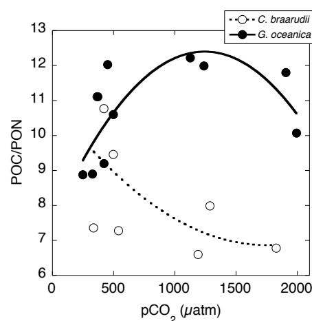
Fig. 4. Evidence for elevated C fixation rates with increasing p\text{CO}_2 in G. oceanica (black circles) arises from elevated POC/PON ratios with increasing p\text{CO}_2 . By contrast, C. braarudii (open circles) appears detrimentally affected, showing a decrease in POC/PON with increasing p\text{CO}_2 .
