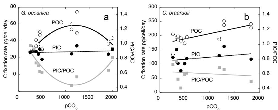
Fig. 3. POC (open circles), PIC (black circles) C fixation rates in pg/cell/day and PIC/POC ratio (grey squares) for G. oceanica with increasing p\text{CO}_2 . Like the earlier experiments of changing pH by Riebesell et al. (2000), there is a decrease in PIC/POC for G. oceanica with increasing p\text{CO}_2 but this is driven by the greater increase in POC relative to the nominal change in calcite production rates. We have plotted a 2nd order polynomial curve through the data where appropriate to highlight the trends.
