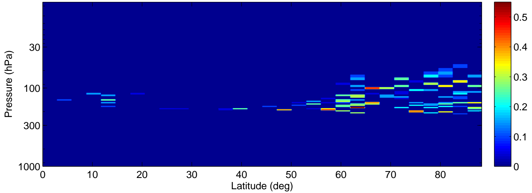
Cloud Water Mixing Ratio (ppmm) for N = 10 \text{ cm}^{-3}
