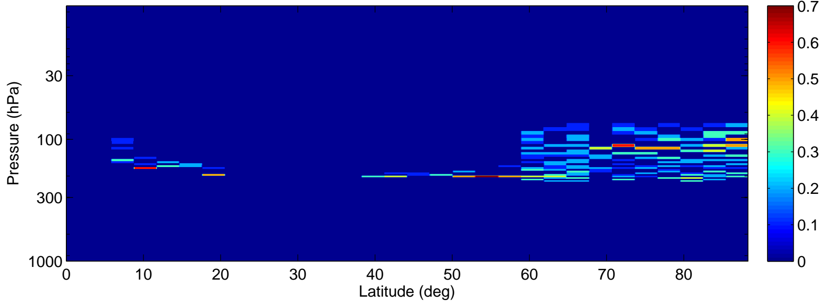
Cloud Water Mixing Ratio (ppmm) for N = 1 \text{ cm}^{-3}
