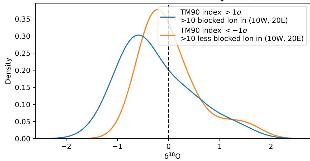
Probability density function of NGT \delta^{18}\text{O} with increased/reduced blocking (TM90)
