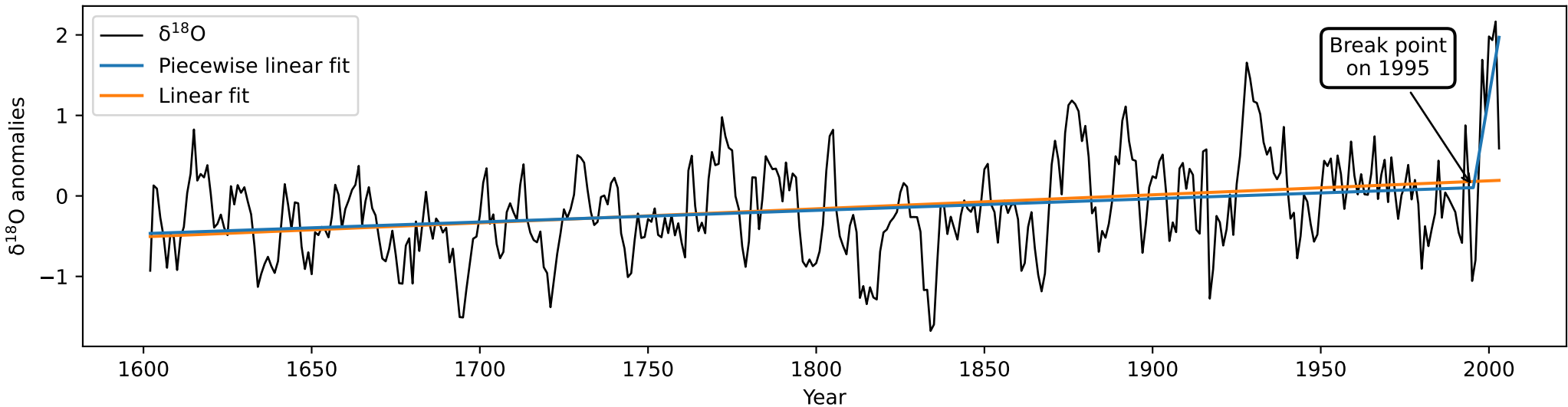
NGT stacked \delta^{18}\text{O} (1602-2003)
