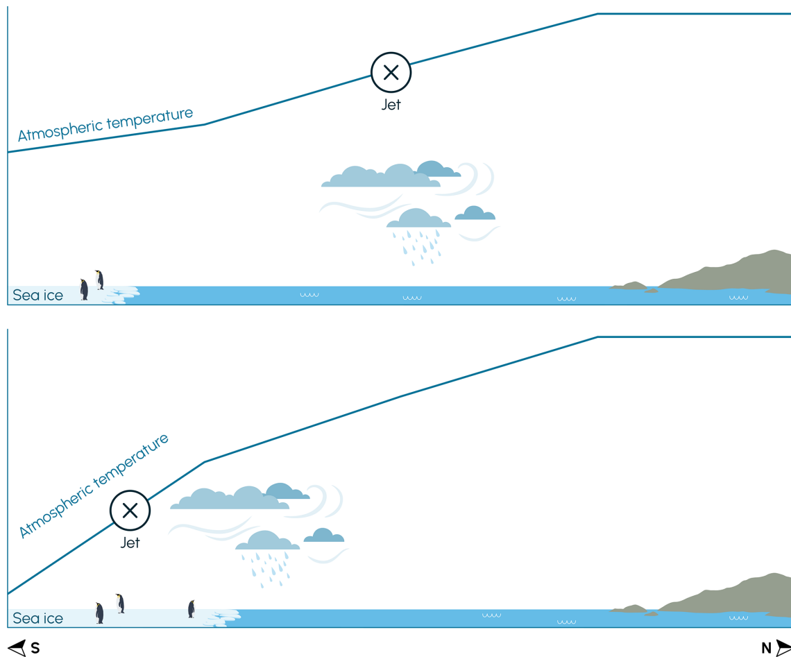
Figure 6. Simplified depiction of the response of the Southern Hemisphere westerly winds to changes in sea-ice extent, which mimics the dynamics of the Southern Annular Mode (SAM). The upper panel depicts a low sea-ice state, or negative SAM anomaly, and the lower panel depicts an expanded sea-ice state, or positive SAM anomaly. The expanded sea ice steepens and shifts poleward the latitudinal temperature gradient between the high and mid latitudes, thus shifting the winds and storm systems south. The jet represents the core of the Southern hemisphere westerly winds, which is associated with the steepest temperature gradient.
