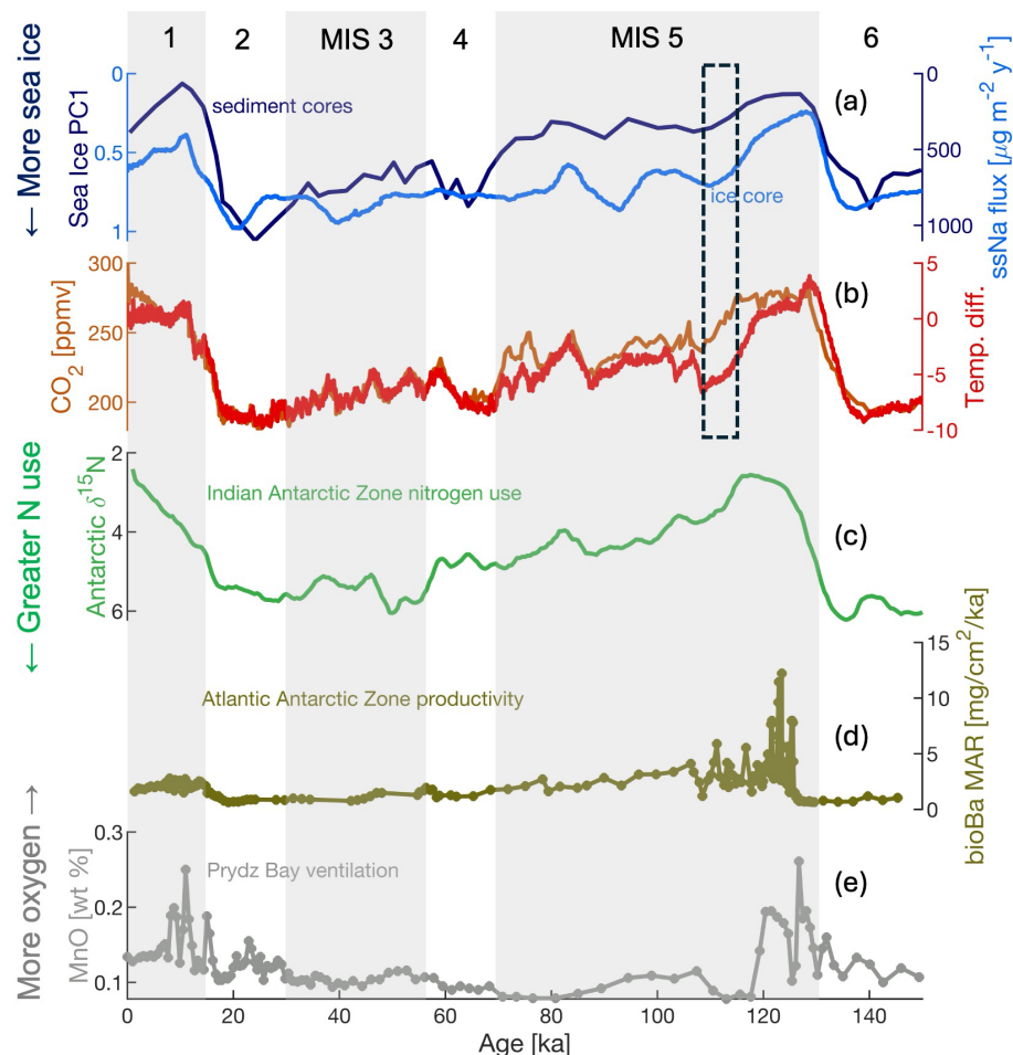
Figure 4. Sea ice and related changes in the Southern Ocean and Antarctica over the past 150 ka. (a) Principal Component 1 of sedimentary sea-ice records (Chadwick et al., 2022c) and the EPICA Dome C sea-ice proxy, ssNa, (Wolff et al., 2010). (b) Antarctic composite CO 2 (Bereiter et al., 2015) and stack of Antarctic surface air temperatures, defined as an anomaly relative to pre-industrial conditions (Parrenin et al., 2013). (c) The mean of the diatom-bound nitrogen isotopic composition from cores MD12-3394 and MD11-3353 from the Antarctic Zone of the Indian Sector (Ai et al., 2020). (d) The biogenic barium flux from ODP 1094/TN67-13PC in the Antarctic Zone of the Atlantic Sector (Jaccard et al., 2013). (e) The weight percent of manganese oxide from core ANT30/P1-02 off Prydz Bay (Wu et al., 2018), an indicator of bottom water ventilation and proxy for AABW formation. Locations of records are shown in Fig. 2. Marine Isotope Stage (MIS) numbers, as indicated by the oxygen isotopic records of marine carbonates (Lisiecki and Raymo, 2005), are listed along the upper x axis. Glacial stages are highlighted by grey vertical bars. The dashed box in panels a and b indicates the period of rapidly decreasing CO 2 during the glacial inception, which occurred after Antarctic surface air temperature started to decrease and after a substantial increase in ssNa flux from the interglacial low.
