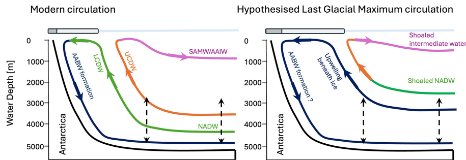
Figure 3. Schematic illustrating the modern Southern Ocean overturning circulation (left) and hypothesised Last Glacial Maximum (LGM) circulation (right). Under present-day conditions, there is mixing (dashed arrows) between the lower branch of the North Atlantic Deep Water (NADW) and the Antarctic Bottom Water (AABW) (vertical arrows). Under conditions of expanded sea-ice extent, the boundary between NADW and AABW shoals, causing less exchange between the two water masses. Greater sea-ice cover particularly in winter (light grey lid) during the LGM is hypothesised to have produced denser bottom waters through more intense brine rejection. The LGM circulation becomes two closed cells rather than the “figure-8” pattern observed in the modern ocean. CDW also upwells mostly under winter sea ice and is transformed into AABW with little air–sea gas exchange (Ferrari et al., 2014). Other water masses pictured are Lower and Upper Circumpolar Deep Water (LCDW and UCDW), Subantarctic Mode Water (SAMW), and Antarctic Intermediate Water (AAIW). Figure after Talley (2013), Sikes et al. (2017), Shub et al. (2024), Hines et al. (2019), and Ronge et al. (2015).
