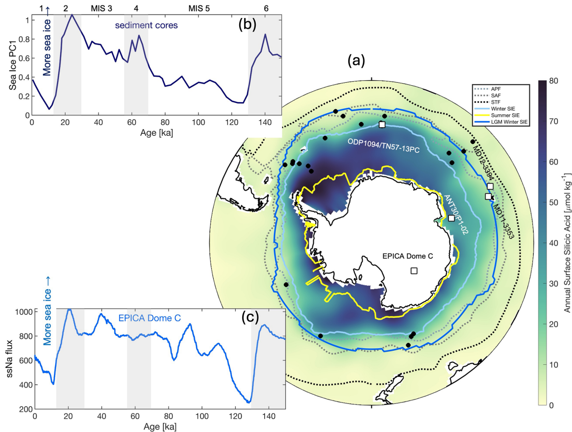
Figure 2. Key Southern Ocean features and proxy records discussed in this paper. (a) Location map showing European Project for Ice Coring in Antarctica (EPICA) Dome C (Wolff et al., 2010), ANT30/P1-02 (Wu et al., 2018), ODP 1094/TN57-13PC (Jaccard et al., 2013), MD11-3353 and MD12-3394 (Ai et al., 2020). The cores used in the sea-ice compilation of Chadwick et al. (2022c) are indicated by black circles. From north to south, the modern locations of the Subtropical Front (STF), Subantarctic Front (SAF) and Antarctic Polar Front (APF) (Orsi et al., 1995) are indicated by dashed grey lines. The modern August (winter) and February (summer) sea-ice edges are shown in light blue and yellow, respectively, derived from the biogeochemical Southern Ocean State Estimate as used in Weis et al. (2024). The estimated August sea-ice edge during the LGM, from Paul et al. (2021), is shown in dark blue. The background colour is the annual average surface silicic acid concentration [ \mu\text{mol kg}^{-1} ] from the World Ocean Atlas (Reagan et al., 2023), showing how this nutrient is “trapped” in the Southern Ocean sea-ice zone. Insets show (b) principal component 1 (PC1) of the sea-ice records from Chadwick et al. (2022c), indicating the dominant temporal trend, and (c) the ice core sea-ice proxy, sea salt sodium (ssNa) flux, in units of \mu\text{g m}^{-2} \text{yr}^{-1} from EPICA Dome C from Wolff et al. (2010).
