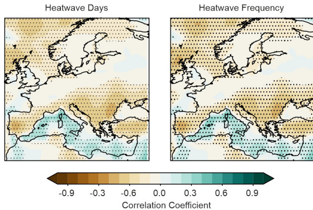
Figure 7. Correlation between ModE-Sim January–May precipitation anomalies (with respect to a 31-year running mean) and June–August heatwave days and frequency. Hatching indicates significant correlations.
