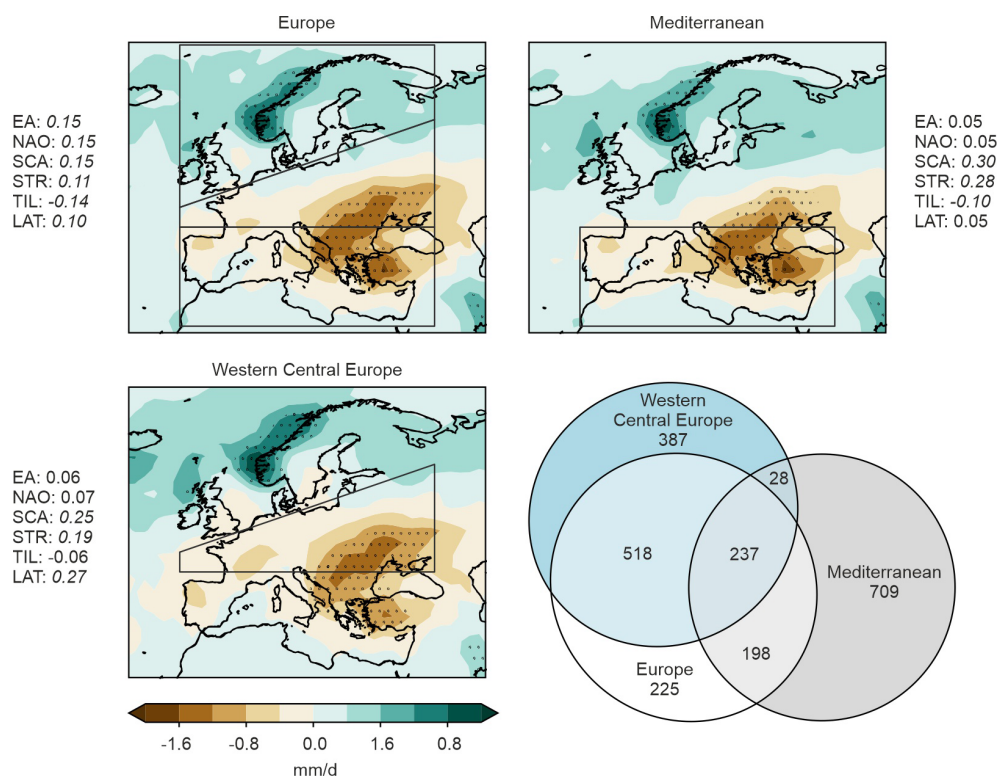
Figure 3. Composites of Mode-RA JFMAM precipitation anomalies for all years and ensemble members with JJA 2 m temperature > 90th percentile in Europe, MED and WCE. Stippling indicates precipitation anomalies larger than two standard deviations. The averages of the six circulation indices, here standardised for better intercomparison are also indicated ( p < 0.05 in italics ). The lower right shows an Euler diagram of the number of cases.
