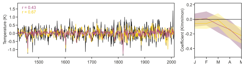
Figure 6. Time series of JJA 2 m temperatures in the land area between 8^{\circ} W and 38^{\circ} E, 36 – 48^{\circ} N in ModeE-RA (black) and predicted from the regression models based on spring-only predictors (purple) and spring-summer predictors (orange). Right: Coefficients (95 % confidence intervals shaded) for precipitation in January to May in the two models.
