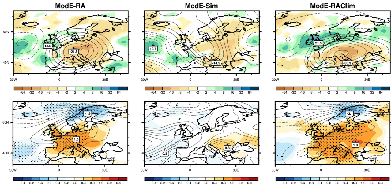
Figure 1. (top) MAM 1473 total precipitation (mm) and SLP anomalies (contour lines) as well as (bottom) JJA 1473 2 m temperature and 500 hPa GPH anomalies (contour lines) for (left) ModE-RA, (middle) ModE-Sim, and (right) ModE-RAclim. Contour distance is 1 hPa for SLP and 10 GPH for 500 hPa GPH (negatives dashed, zero not shown). Stippling indicates where at least 15 out of 20 members agree in sign. Minima and maxima in temperature and precipitation are indicated.
