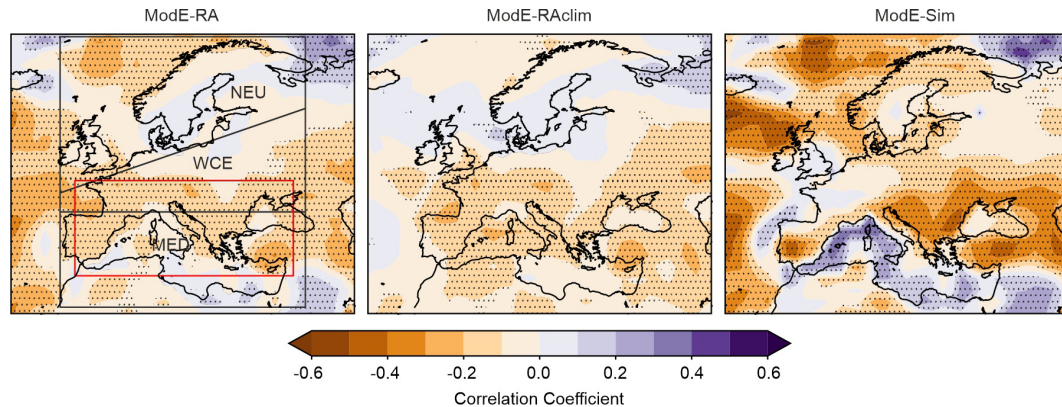
Figure 2. Gridpoint-based correlations between JFMAM precipitation anomalies and JJA 2 m temperature anomalies for (left) ModeE-RA, (middle) ModeE-RAclim, and (right) ModeE-Sim, 1421–2008. Stippling indicates significance at the 95 % confidence level. The left figure shows the IPCC regions NEU, WCE, and MED. The red rectangle shows the region used for the regression approach.
