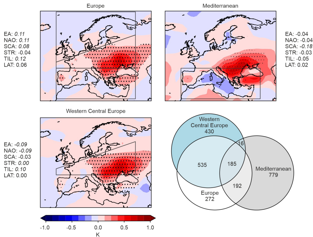
Figure 4. Composites of Mode-RA JJA 2 m temperature anomalies for all years and ensemble members with JFMAM precipitation < 10th percentile in Europe, MED, and WCE. Stippling indicates 2 m temperature anomalies exceeding two standard deviations. The averages of the six circulation indices, here standardised for better intercomparison are also indicated ( p < 0.05 in italics). The lower right shows an Euler diagram of the number of the cases.
