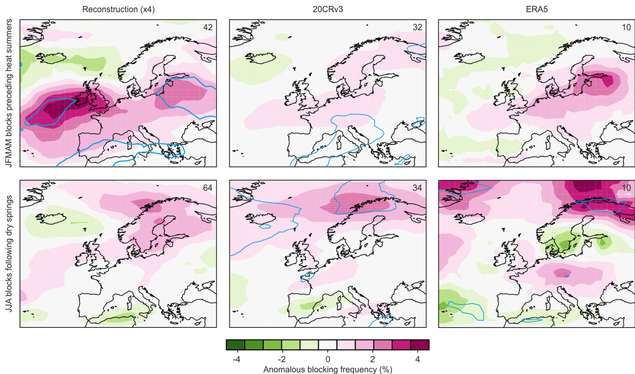
Figure 5. Anomalies in blocking in JFMAM preceding heat summers in Europe (top) and in JJA following dry springs in Europe (bottom) in three different data sets (left to right). Blue lines indicate significant ( p < 0.05 , t -test) anomalies. Numbers in the top left indicate the spatial average of blocking (italics indicate significance), and the number of cases is indicated in the top right.
